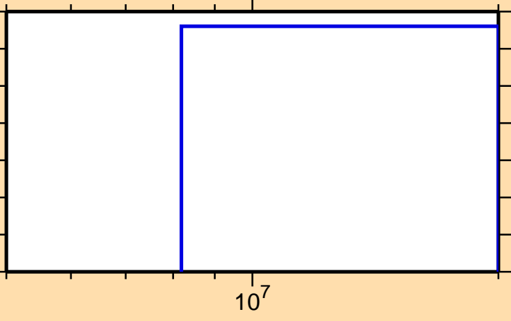
\sigma vs. E for ^{132}\text{Sb}(n,2np)
