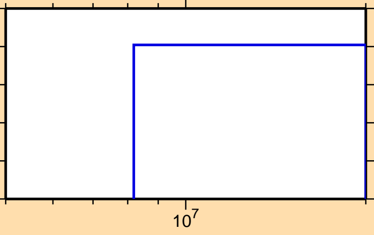
\sigma vs. E for ^{132}\text{Sb}(n,np)
