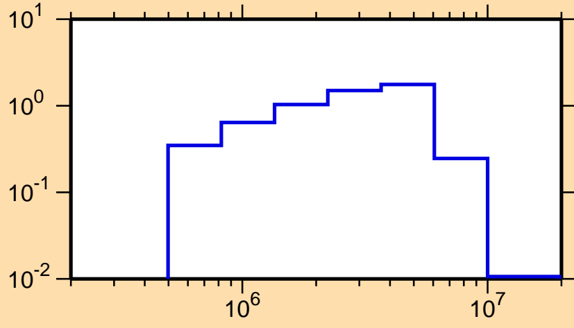
\sigma vs. E for ^{134}\text{Sb}(n,\text{inel.})
