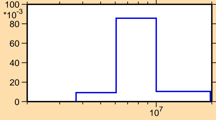
\sigma vs. E for ^{134}\text{Sb}(n,n\text{cont.})
