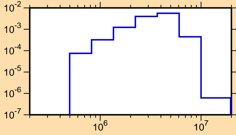
\sigma vs. E for ^{134}\text{Sb}(n,n_1)
