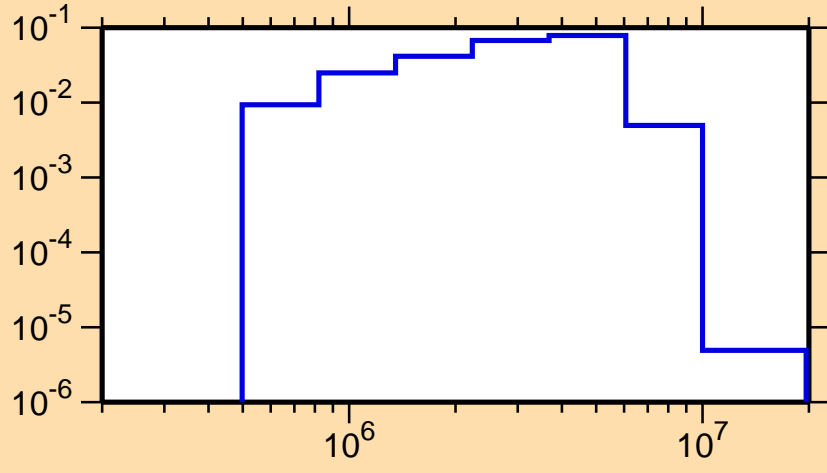
\sigma vs. E for ^{134}\text{Sb}(n,n_4)
