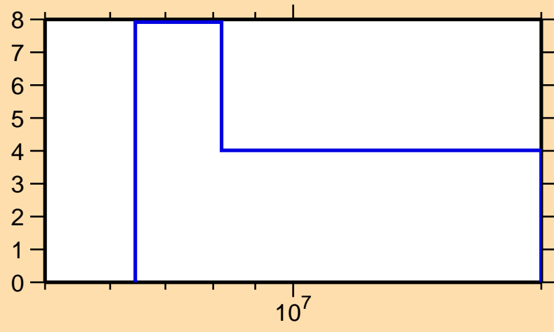
\Delta\sigma/\sigma vs. E for ^{134}\text{Sb}(n,\text{tot.})
