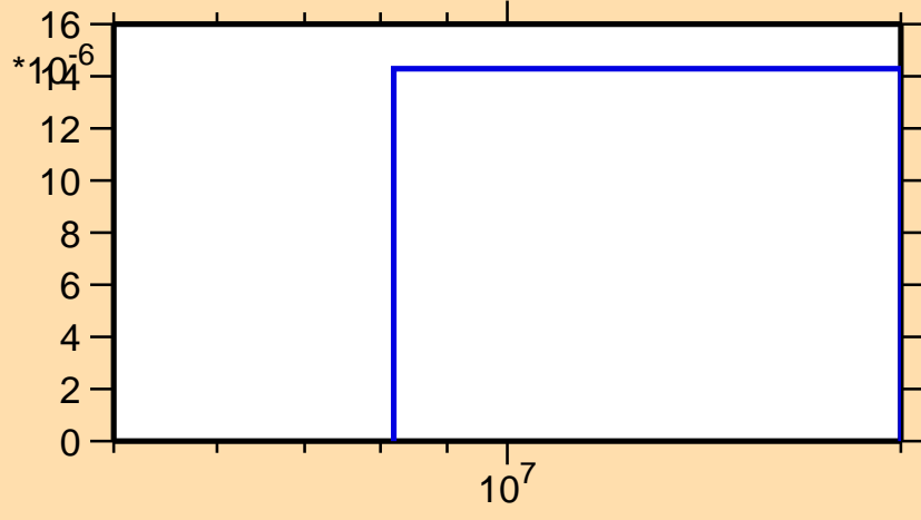
\sigma vs. E for ^{134}\text{Sb}(n,np)
