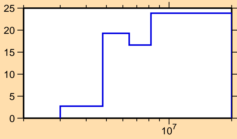
\Delta\sigma/\sigma vs. E for ^{134}\text{Sb}(n,2n)
