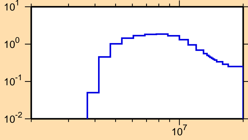
\sigma vs. E for ^{135}\text{Sb}(n,2n)
