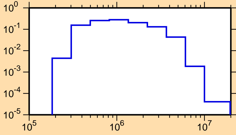
\sigma vs. E for ^{135}\text{Sb}(n,n_1)
