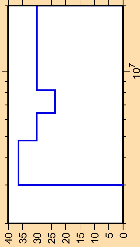
\Delta\sigma/\sigma vs. E for ^{135}\text{Sb}(n,ncont.)
