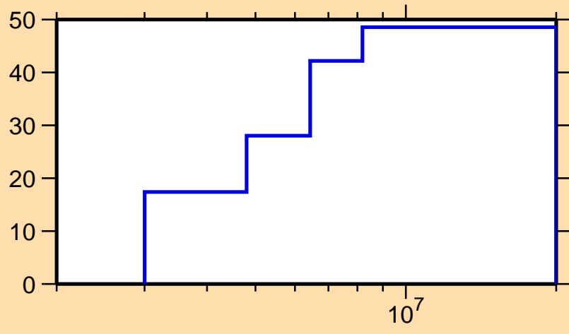
\Delta\sigma/\sigma vs. E for ^{135}\text{Sb}(n,inel.)
