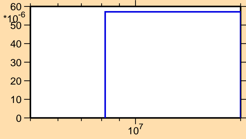
\sigma vs. E for ^{135}\text{Sb}(n,p)
