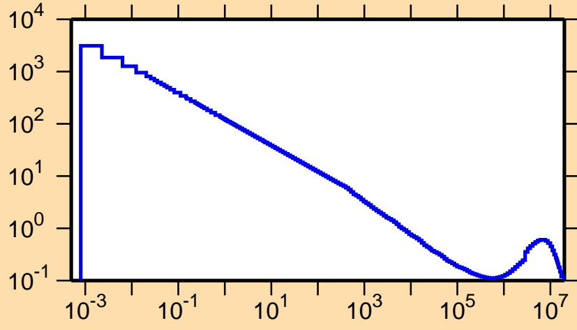
\sigma vs. E for ^{42}\text{Sc}(n,\alpha)
