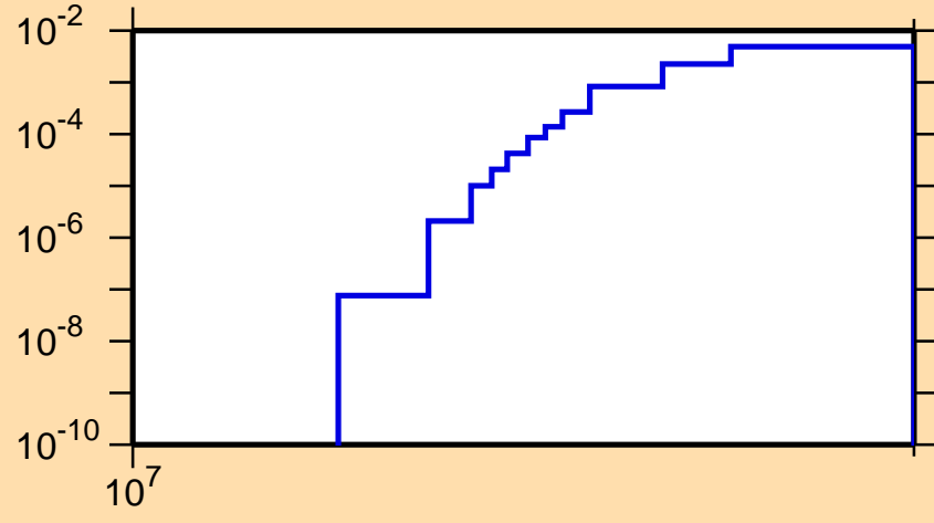
\sigma vs. E for ^{42}\text{Sc}(n,pd)
