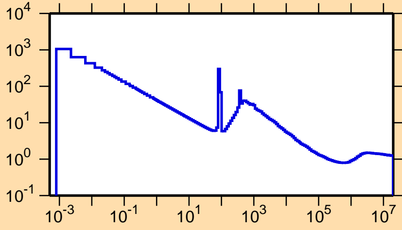
\sigma vs. E for ^{43}\text{Sc}(n,\text{nonel.})
