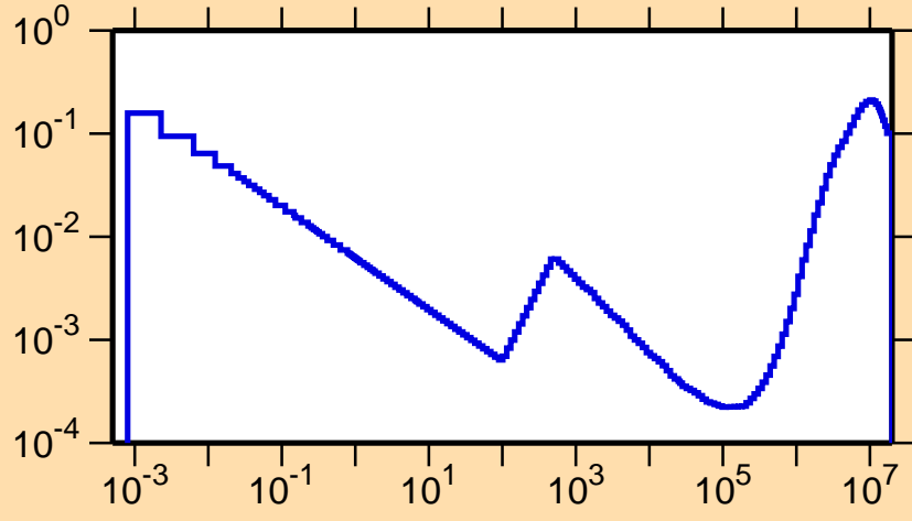
\sigma vs. E for ^{43}\text{Sc}(n,\alpha)
