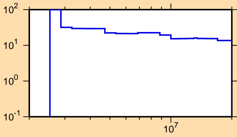
\Delta\sigma/\sigma vs. E for ^{43}\text{Sc}(n,ncont.)
