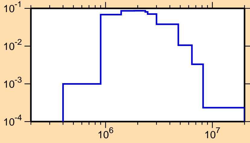
\sigma vs. E for ^{43}\text{Sc}(n,n_3)
