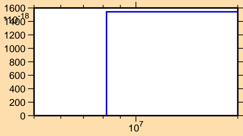
\sigma vs. E for ^{43}\text{Sc}(\text{mt } 34)
