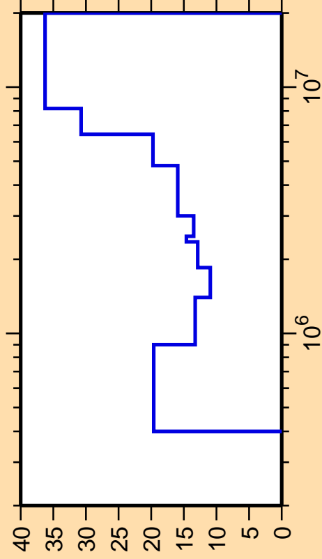
\Delta\sigma/\sigma vs. E for ^{43}\text{Sc}(n,n_3)
