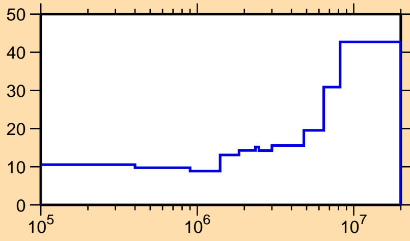
\Delta\sigma/\sigma vs. E for ^{43}\text{Sc}(n,n_1)
