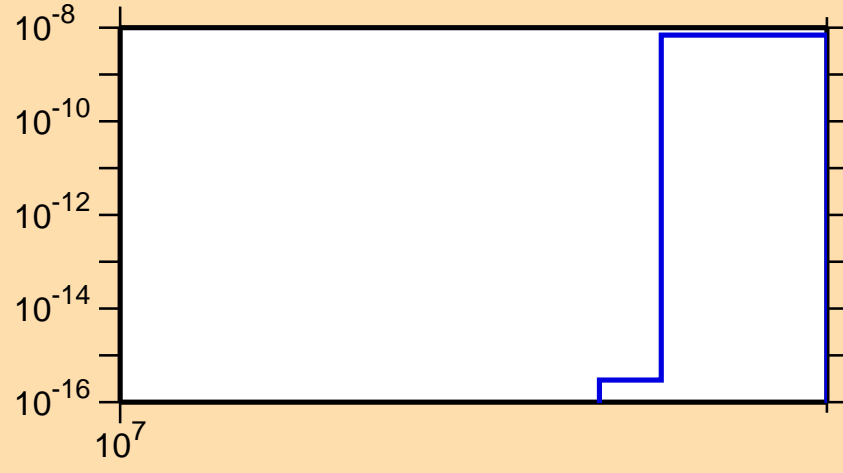
\sigma vs. E for ^{44}\text{Sc}(n,pd)
