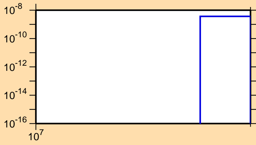
\sigma vs. E for ^{44}\text{Sc} (mt 45)
