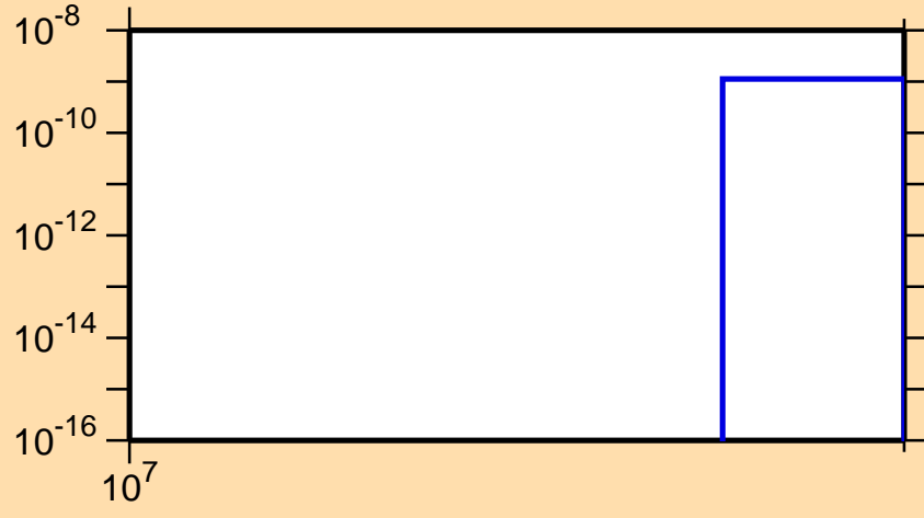
\sigma vs. E for ^{44}\text{Sc}(n,\text{pt})
