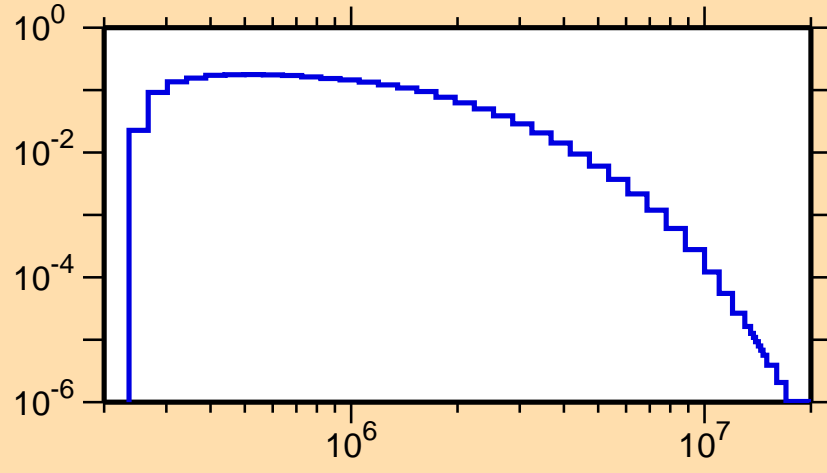
\sigma vs. E for ^{44}\text{Sc}(n,n_3)
