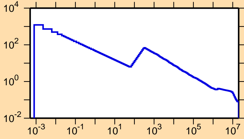
\sigma vs. E for ^{44}\text{Sc}(n,p)
