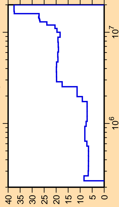
\Delta\sigma/\sigma vs. E for ^{44}\text{Sc}(n,n_3)
