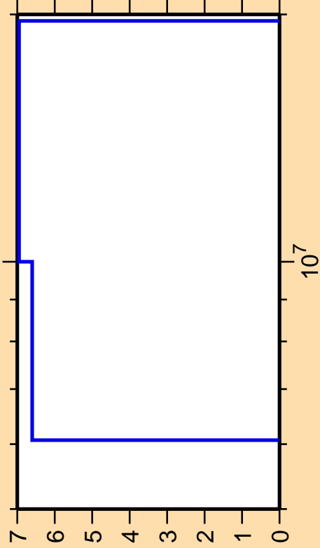
\Delta\sigma/\sigma vs. E for ^{45}\text{Sc}(n,np)
