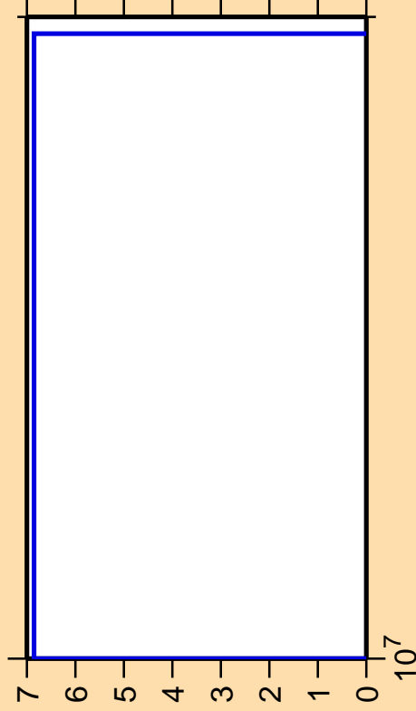
\Delta\sigma/\sigma vs. E for ^{45}\text{Sc}(n,2n)
