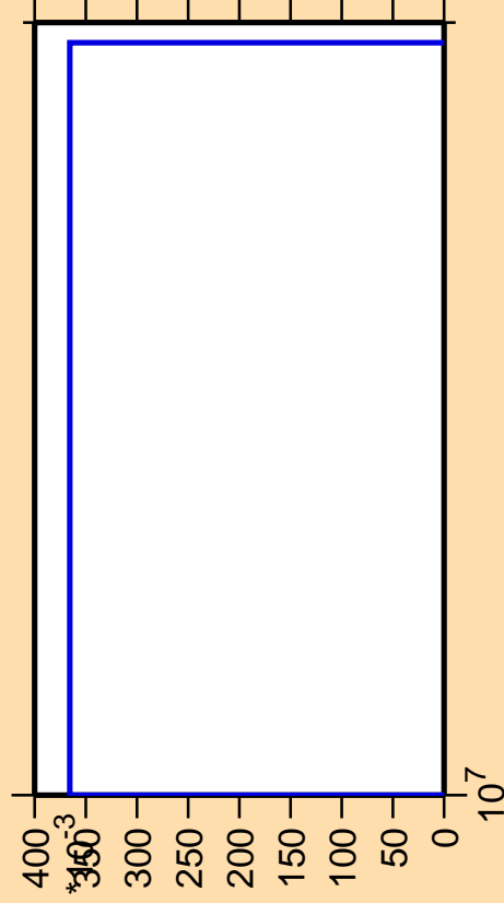
\Delta\sigma/\sigma vs. E for ^{45}\text{Sc}(\text{mt117})
