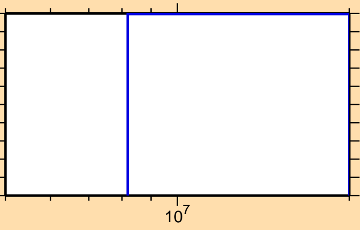
\sigma vs. E for ^{47}\text{Sc}(n,t)
