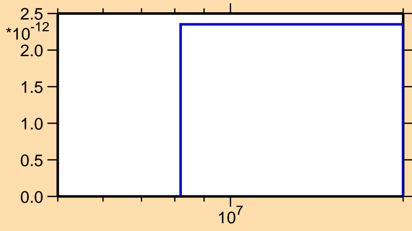
\sigma vs. E for ^{47}\text{Sc}(n,nt)
