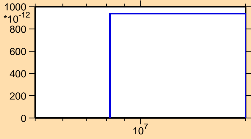
\sigma vs. E for ^{47}\text{Sc}(n,3n)
