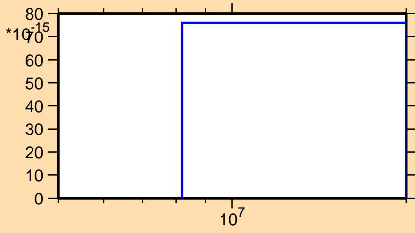
\sigma vs. E for ^{47}\text{Sc}(n,2np)
