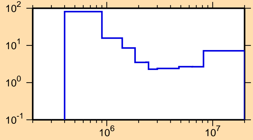
\Delta\sigma/\sigma vs. E for ^{47}\text{Sc}(n,\text{inel.})
