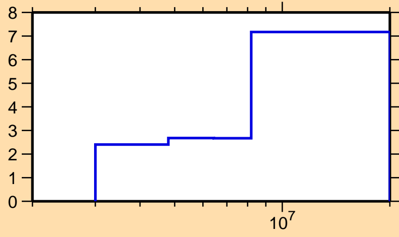
\Delta\sigma/\sigma vs. E for ^{47}\text{Sc}(n,\text{inel.})
