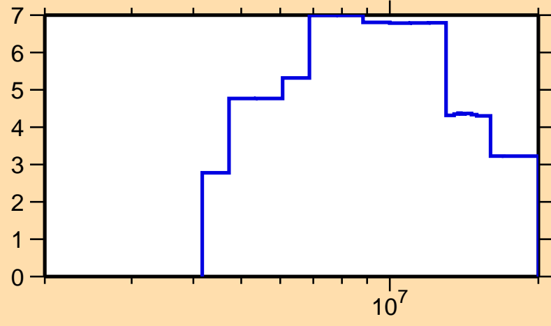
\Delta\sigma/\sigma vs. E for ^{49}\text{Sc}(n,el.)
