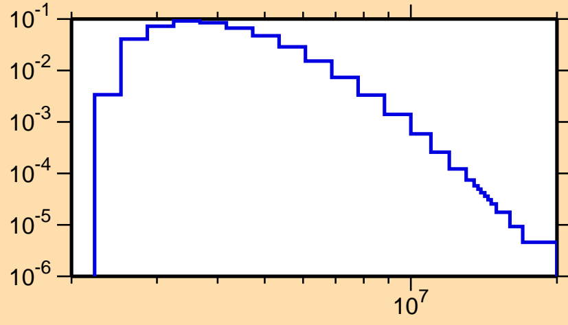
\sigma vs. E for ^{49}\text{Sc}(n,n_2)
