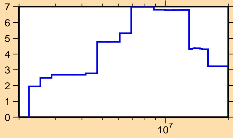
\Delta\sigma/\sigma vs. E for ^{49}\text{Sc}(n,\text{el.})
