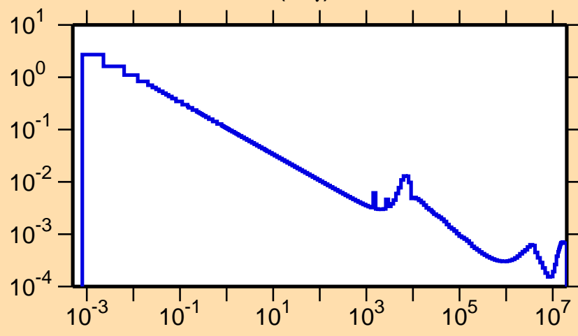
\sigma vs. E for ^{49}\text{Sc}(n,\gamma)
