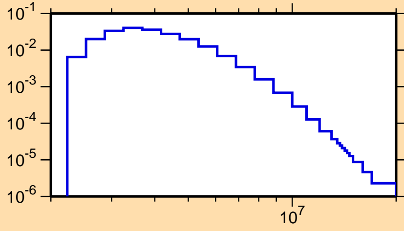
\sigma vs. E for ^{49}\text{Sc}(n,n_1)
