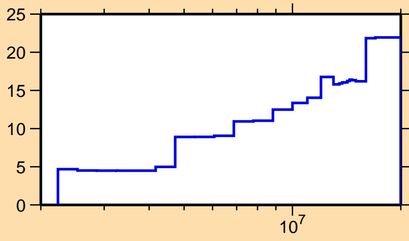
\Delta\sigma/\sigma vs. E for ^{49}\text{Sc}(n,n_1)
