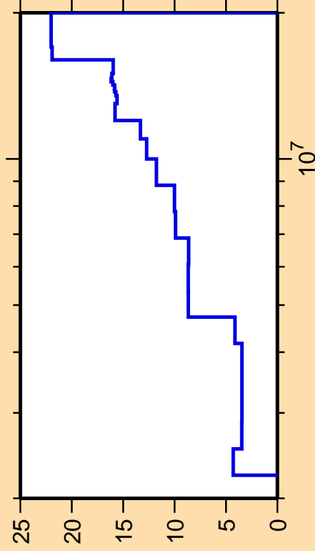
\Delta\sigma/\sigma vs. E for ^{49}\text{Sc}(n,n_2)
