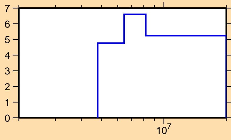
\Delta\sigma/\sigma vs. E for ^{49}\text{Sc}(n,\text{el.})
