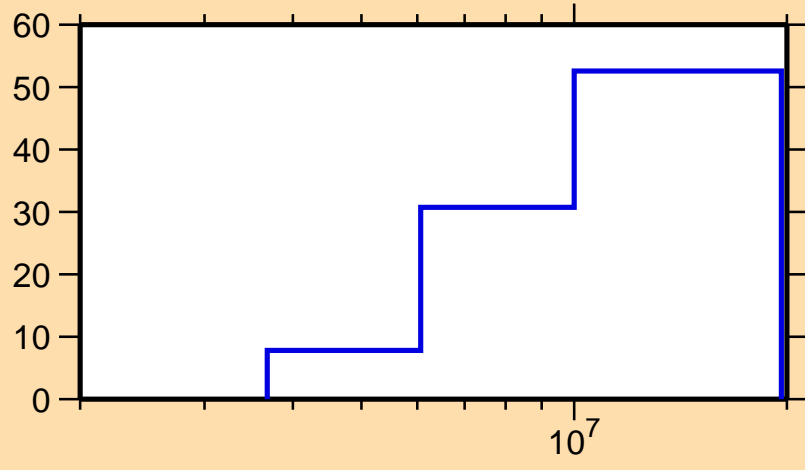
\Delta\sigma/\sigma vs. E for ^{50}\text{Sc}(n,n_1)
