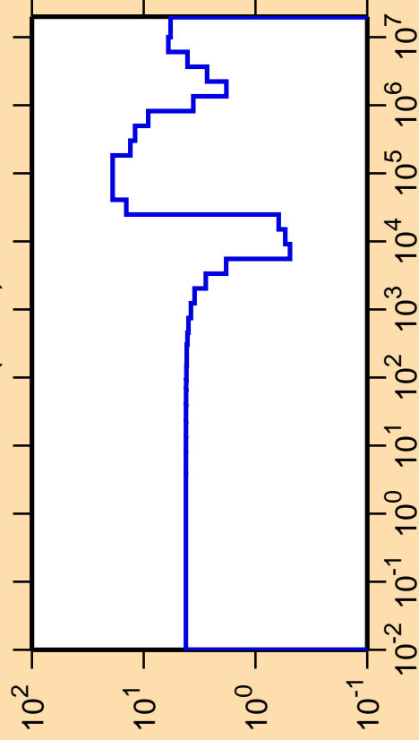
\Delta\sigma/\sigma vs. E for ^{50}\text{Sc}(n,\text{el.})
