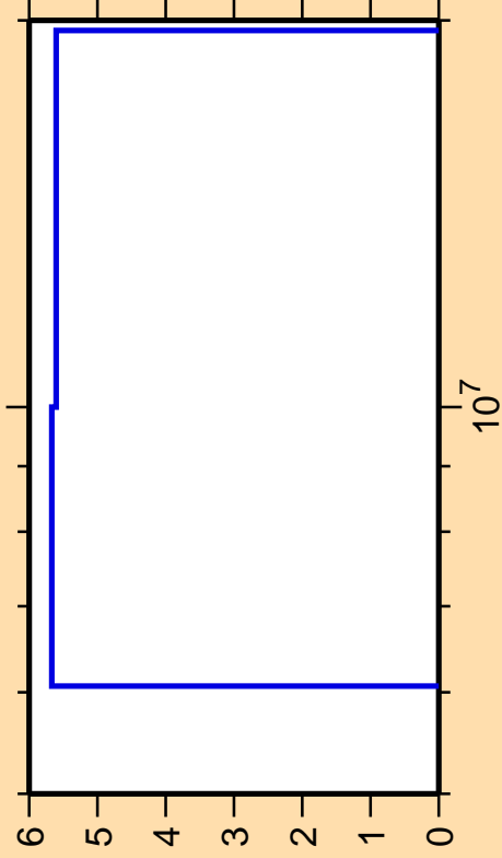
\Delta\sigma/\sigma vs. E for ^{50}\text{Sc}(n,2n)
