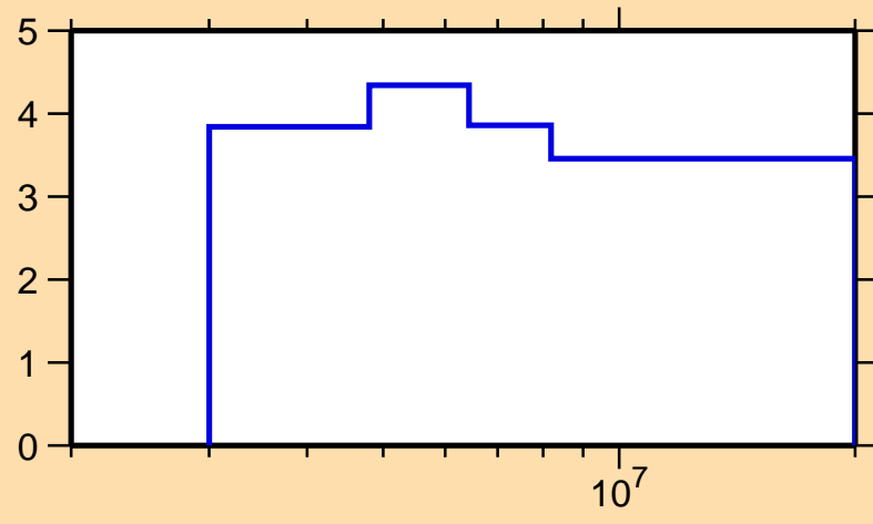
\Delta\sigma/\sigma vs. E for ^{50}\text{Sc}(n,n\text{onel.})
