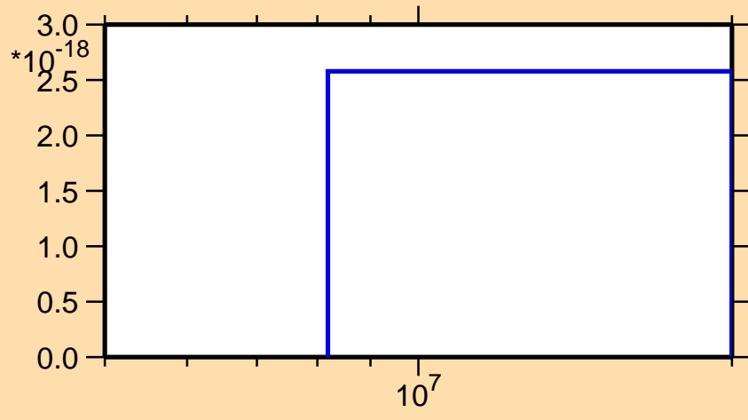
\sigma vs. E for ^{50}\text{Sc}(n,2n\alpha)
