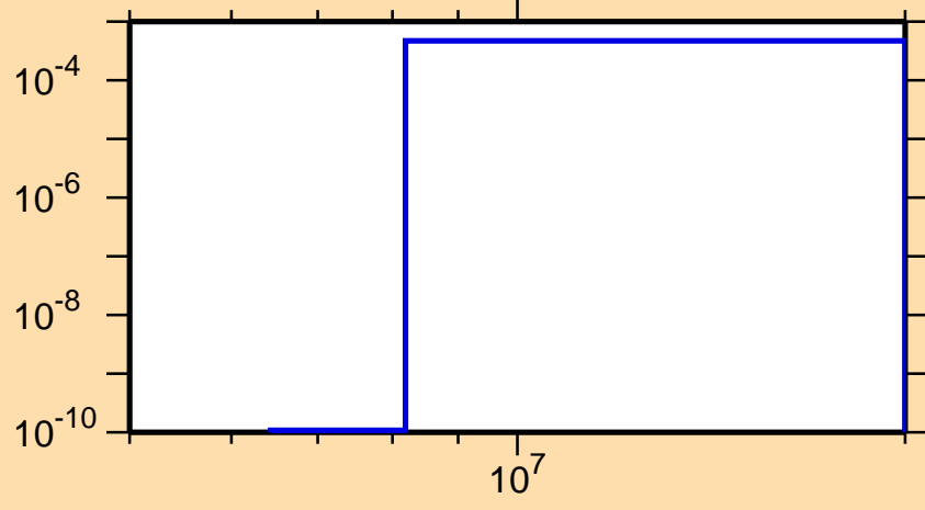
\sigma vs. E for ^{51}\text{Sc}(n,\alpha)
