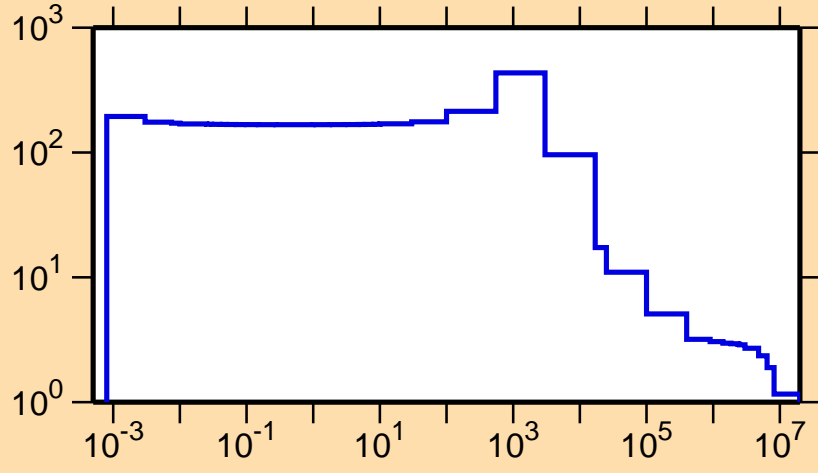
\sigma vs. E for ^{51}\text{Sc}(n,\text{el.})
