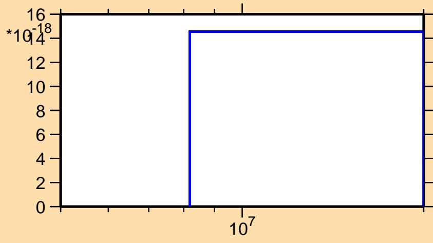
\sigma vs. E for ^{51}\text{Sc}(n,2n\alpha)
