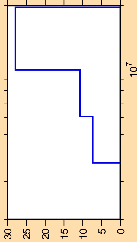
\Delta\sigma/\sigma vs. E for ^{52}\text{Sc}(n,n\text{cont.})
