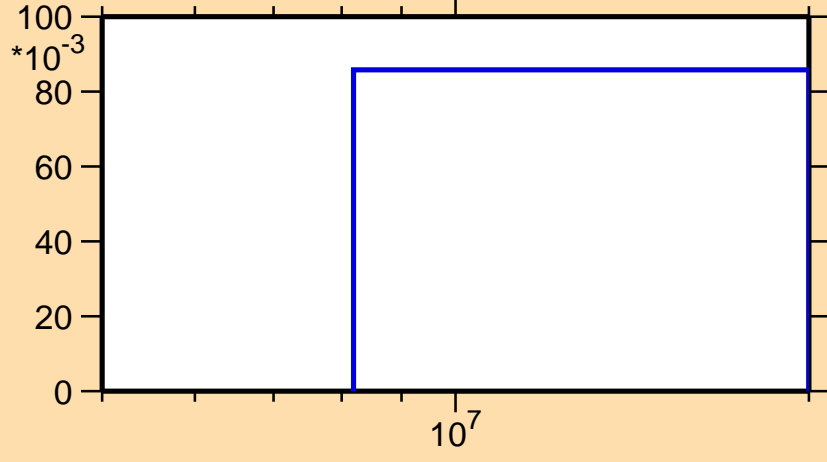
\sigma vs. E for ^{52}\text{Sc}(n,3n)
