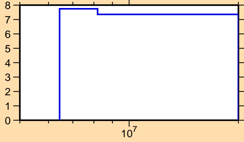
\Delta\sigma/\sigma vs. E for ^{52}\text{Sc}(n,2n)
