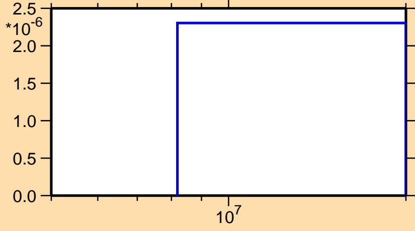
\sigma vs. E for ^{52}\text{Sc}(n,n\alpha)
