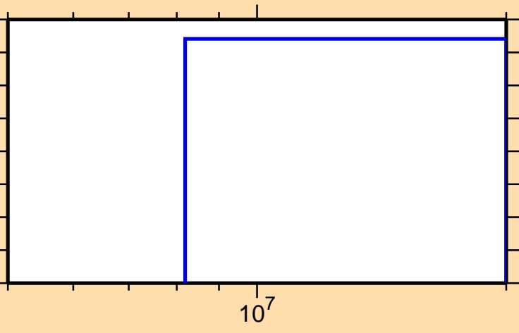
\sigma vs. E for ^{53}\text{Sc}(n,\alpha)
