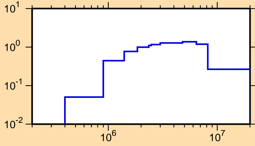
\sigma vs. E for ^{53}\text{Sc}(n,n\text{cont.})
