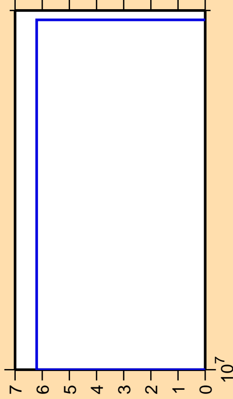
\Delta\sigma/\sigma vs. E for ^{68}\text{Se} (mt 34)
