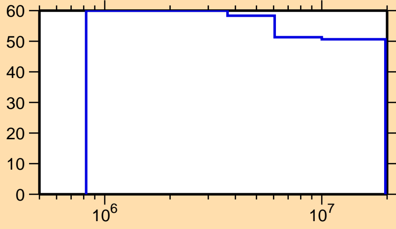
\Delta\sigma/\sigma vs. E for ^{68}\text{Se}(n,n_1)
