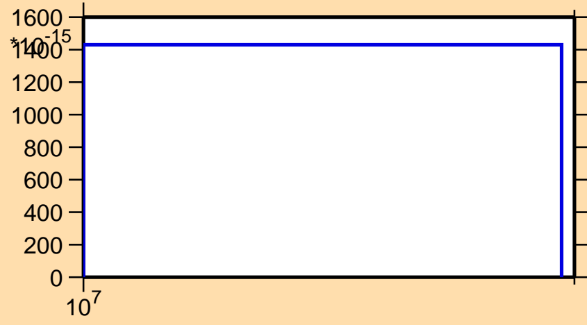
\sigma vs. E for ^{68}\text{Se} (mt 34)
