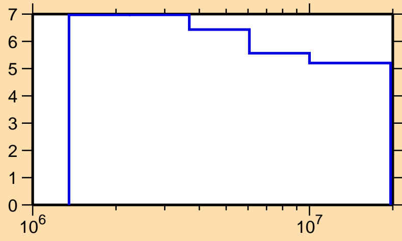
\Delta\sigma/\sigma vs. E for ^{68}\text{Se}(n,\text{nonel.})
