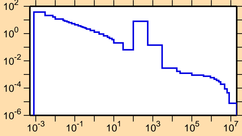
\sigma vs. E for ^{68}\text{Se}(n,\gamma)
