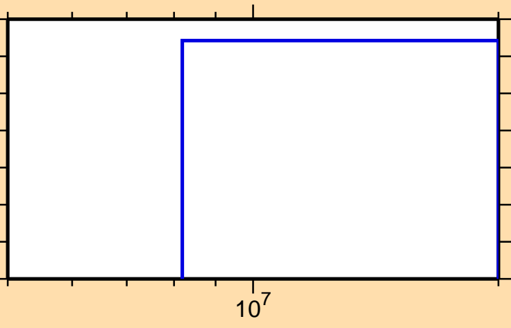
\sigma vs. E for ^{68}\text{Se}(n,2np)
