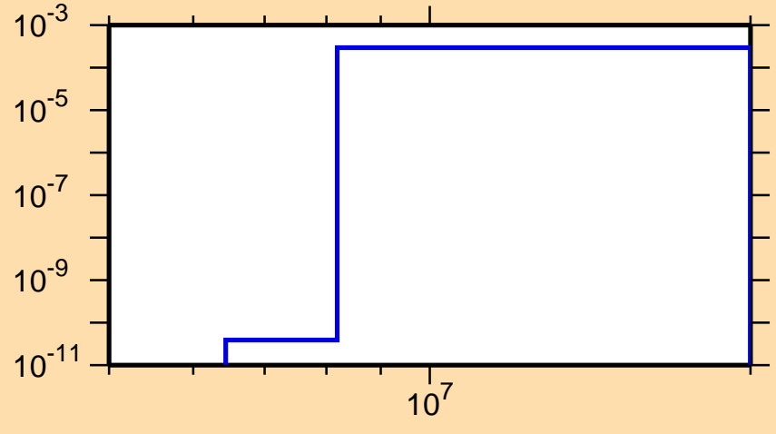
\sigma vs. E for ^{68}\text{Se}(n,pd)
