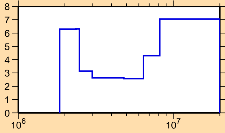
\Delta\sigma/\sigma vs. E for ^{68}\text{Se}(n,\text{tot.})
