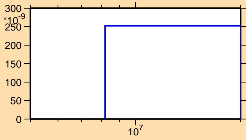
\sigma vs. E for ^{68}\text{Se}(n,t)
