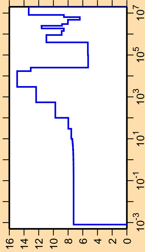
\Delta\sigma/\sigma vs. E for ^{68}\text{Se}(n,\text{el.})
