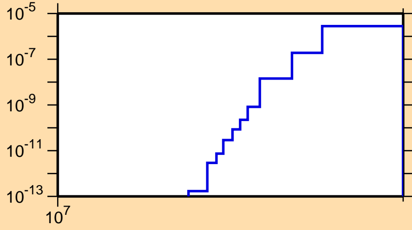
\sigma vs. E for ^{69}\text{Se} (mt 34)
