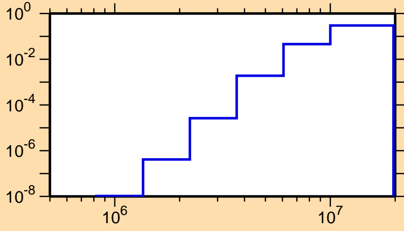
\sigma vs. E for ^{69}\text{Se}(n,p\alpha)
