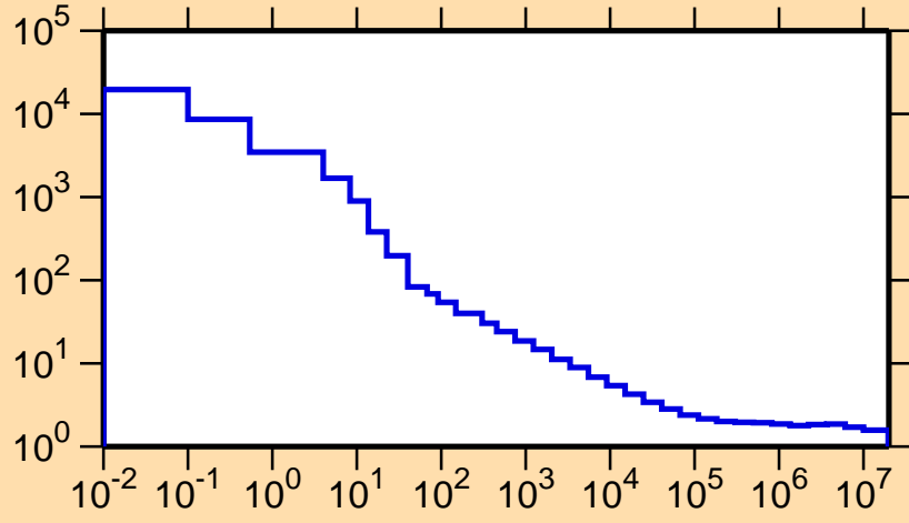
\sigma vs. E for ^{69}\text{Se}(n,\text{nonel.})
