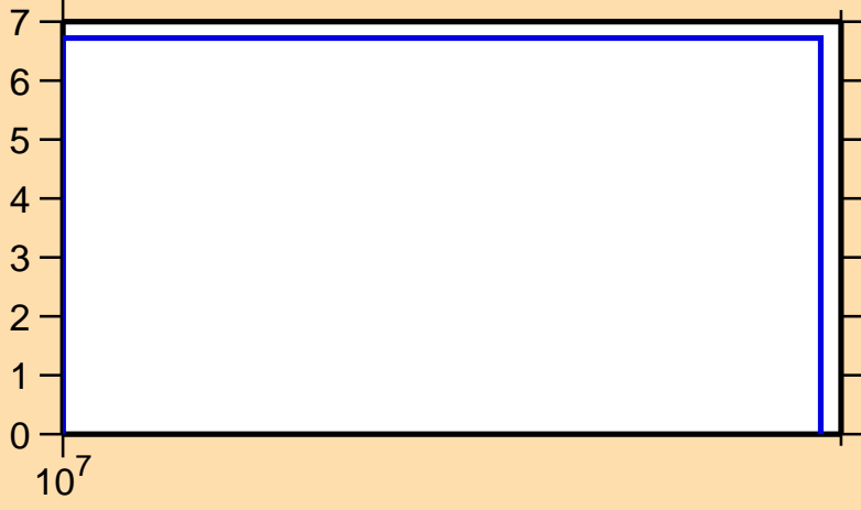
\Delta\sigma/\sigma vs. E for ^{69}\text{Se}(n,\text{el.})
