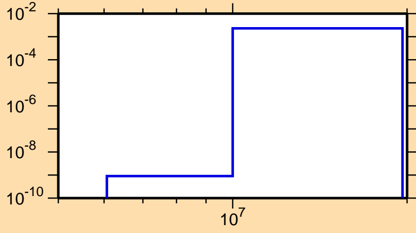
\sigma vs. E for ^{69}\text{Se}(n,pd)
