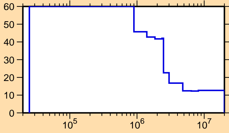
\Delta\sigma/\sigma vs. E for ^{69}\text{Se}(n,n_1)
