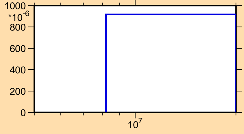
\sigma vs. E for ^{69}\text{Se}(n,2n)
