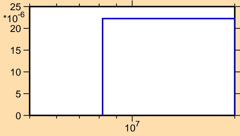
\sigma vs. E for ^{69}\text{Se}(n,\text{pt})
