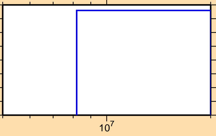
\sigma vs. E for ^{69}\text{Se}(n,nt)
