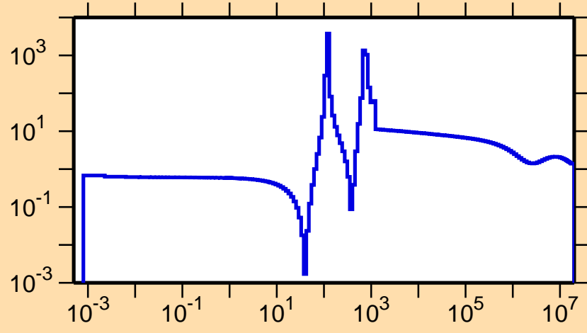
\sigma vs. E for ^{70}\text{Se}(n,\text{el.})
