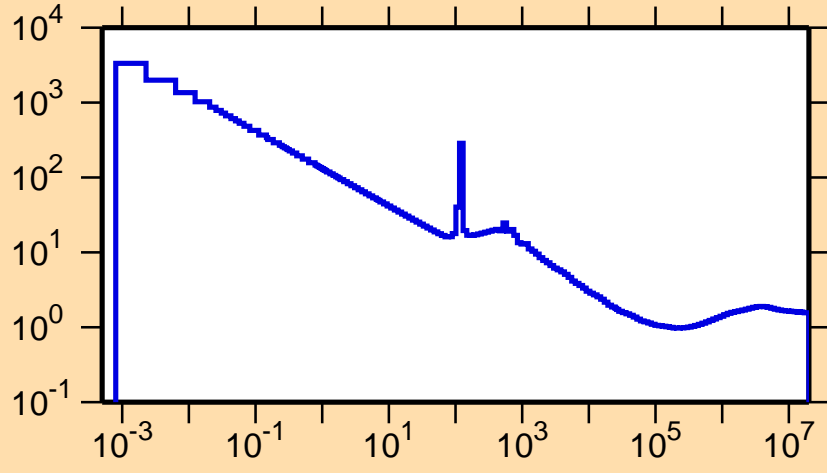
\sigma vs. E for ^{70}\text{Se}(n,\text{nonel.})
