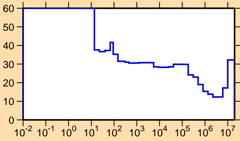
\Delta\sigma/\sigma vs. E for ^{70}\text{Se}(n,p)
