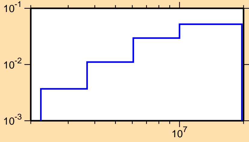
\sigma vs. E for ^{70}\text{Se}(n,n\text{cont.})
