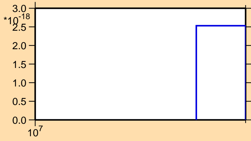
\sigma vs. E for ^{71}\text{Se}(n,nt)
