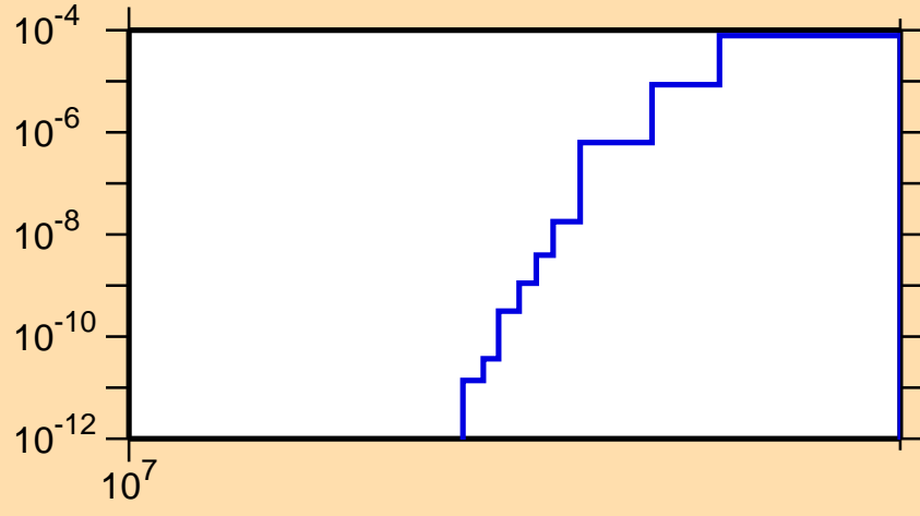
\sigma vs. E for ^{71}\text{Se}(n,pt)
