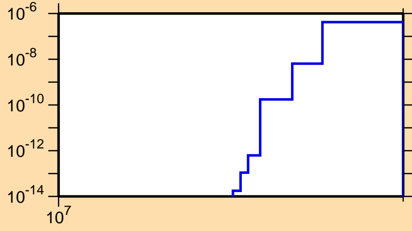
\sigma vs. E for ^{71}\text{Se} (mt 34)
