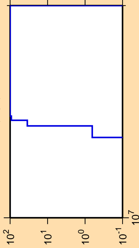
\Delta\sigma/\sigma vs. E for ^{71}\text{Se}(n,pt)
