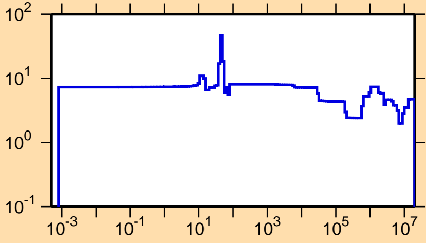
\Delta\sigma/\sigma vs. E for ^{71}\text{Se}(n,el.)
