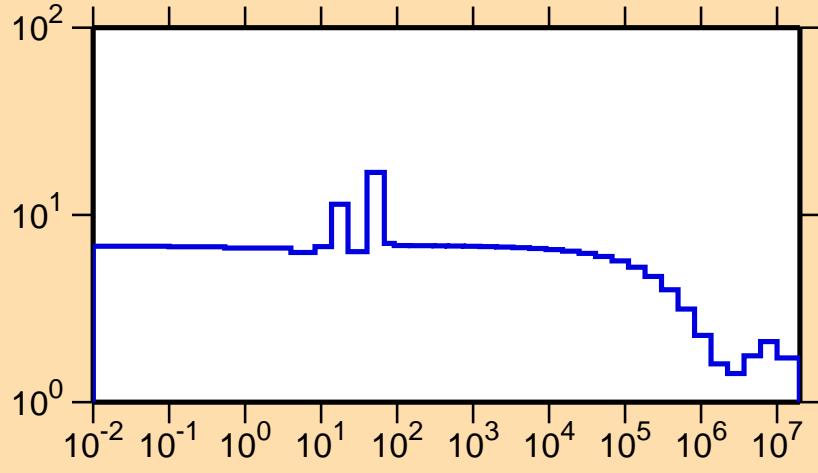
\sigma vs. E for ^{71}\text{Se}(n,\text{el.})
