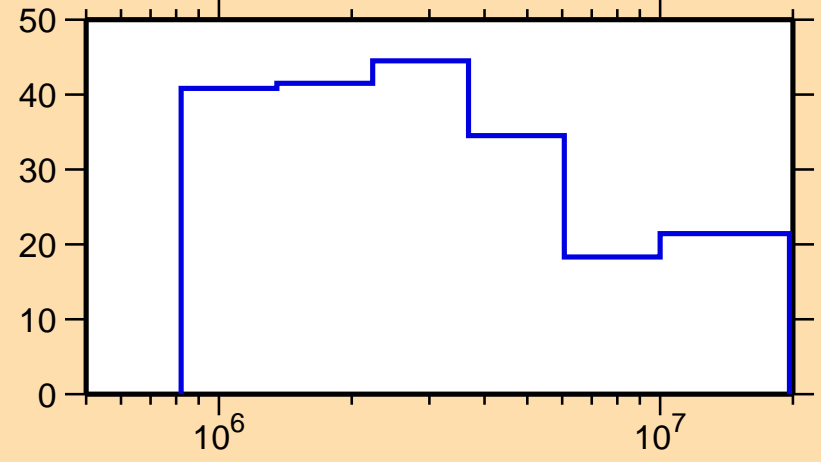
\Delta\sigma/\sigma vs. E for ^{71}\text{Se}(n,ncont.)
