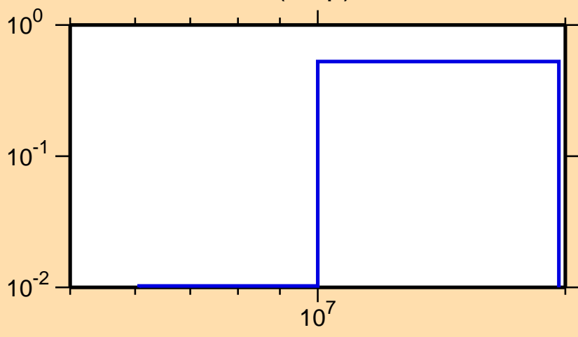
\sigma vs. E for ^{71}\text{Se}(n,np)
