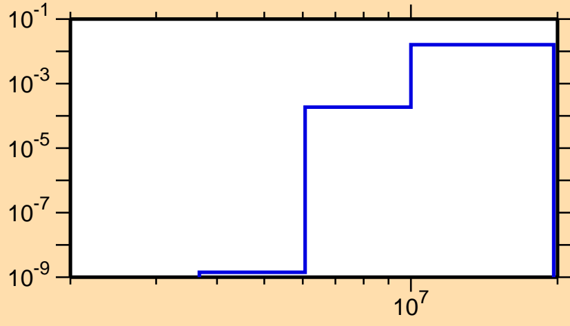
\sigma vs. E for ^{71}\text{Se}(n,d)
