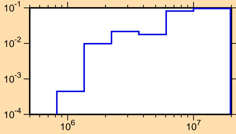
\sigma vs. E for ^{71}\text{Se}(n,n\text{cont.})
