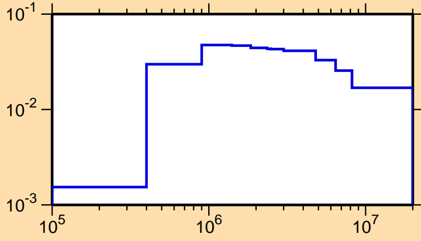
\sigma vs. E for ^{71}\text{Se}(n,n_4)
