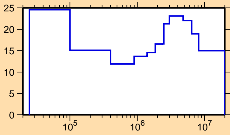
\Delta\sigma/\sigma vs. E for ^{71}\text{Se}(n,n_1)
