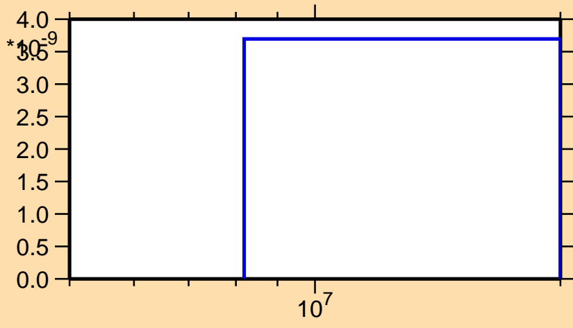
\sigma vs. E for ^{71}\text{Se} (mt 34)
