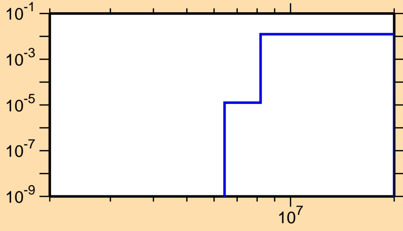
\sigma vs. E for ^{71}\text{Se}(n,n\alpha)
