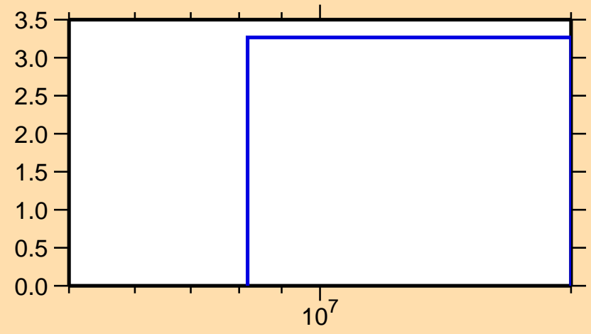
\Delta\sigma/\sigma vs. E for ^{71}\text{Se}(n,\text{nonel.})
