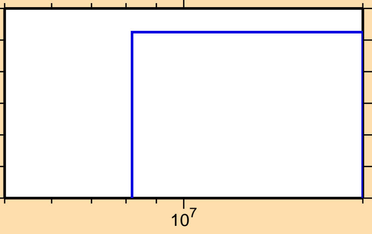
\sigma vs. E for ^{71}\text{Se}(n,\text{pd})
