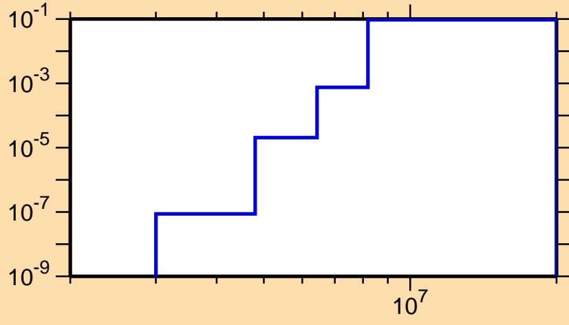
\sigma vs. E for ^{71}\text{Se}(n,p\alpha)
