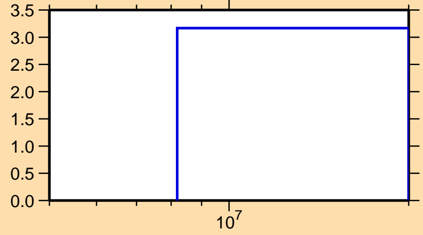
\Delta\sigma/\sigma vs. E for ^{71}\text{Se}(n,\text{tot.})
