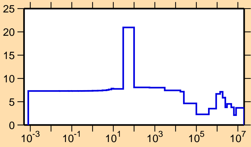
\Delta\sigma/\sigma vs. E for ^{71}\text{Se}(n,\text{el.})
