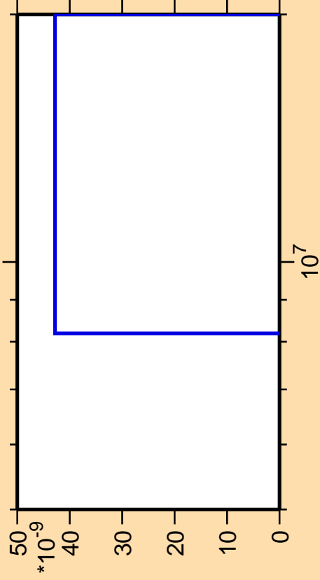
\Delta\sigma/\sigma vs. E for ^{71}\text{Se}(n,nt)
