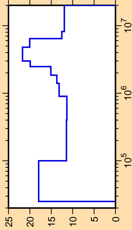
\Delta\sigma/\sigma vs. E for ^{71}\text{Se}(n,\text{inel.})
