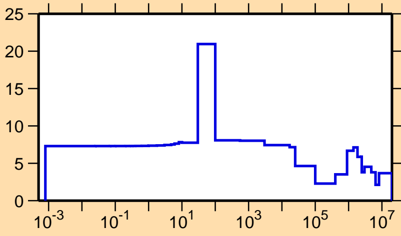
\Delta\sigma/\sigma vs. E for ^{71}\text{Se}(n,el.)
