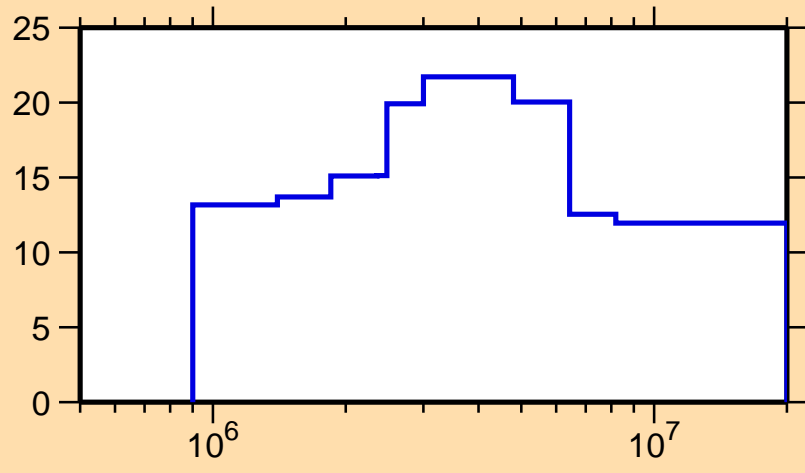
\Delta\sigma/\sigma vs. E for ^{71}\text{Se}(n,\text{inel.})
