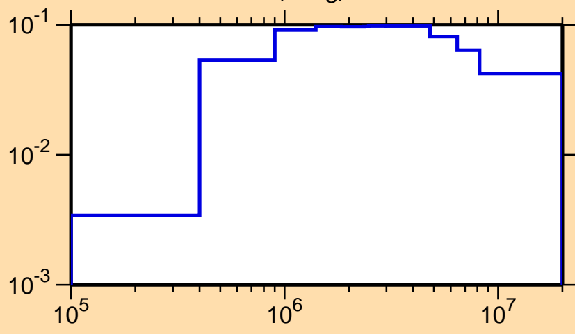
\sigma vs. E for ^{71}\text{Se}(n,n_3)
