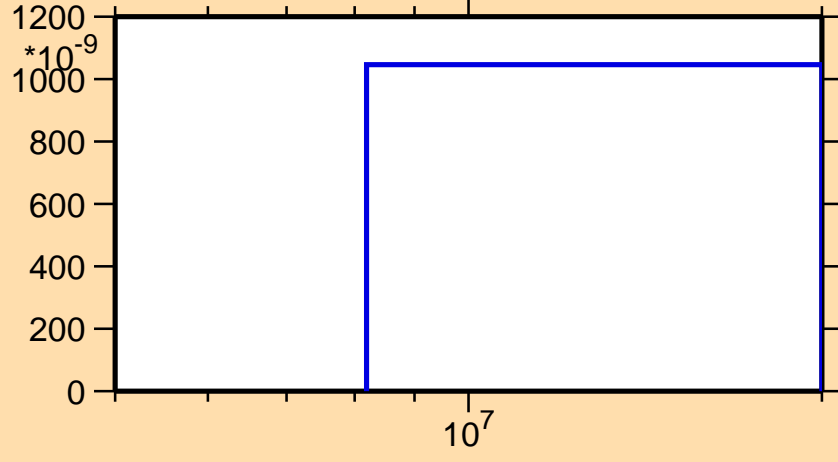
\sigma vs. E for ^{71}\text{Se}(n,pt)
