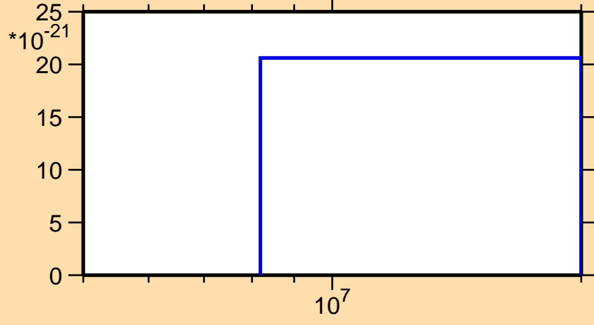
\sigma vs. E for ^{71}\text{Se}(n,nt)
