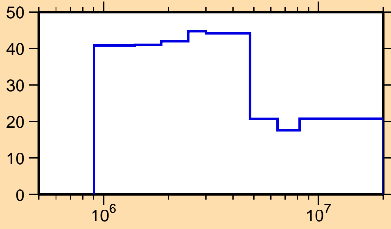
\Delta\sigma/\sigma vs. E for ^{71}\text{Se}(n,n\text{cont.})
