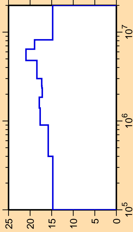
\Delta\sigma/\sigma vs. E for ^{71}\text{Se}(n,n_2)
