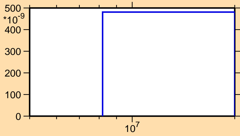
\sigma vs. E for ^{71}\text{Se}(n,2np)
