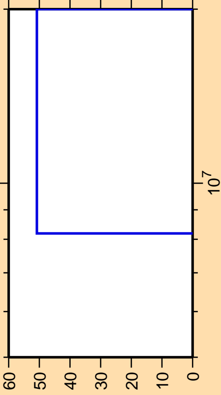
\Delta\sigma/\sigma vs. E for ^{71}\text{Se}(n,2n)
