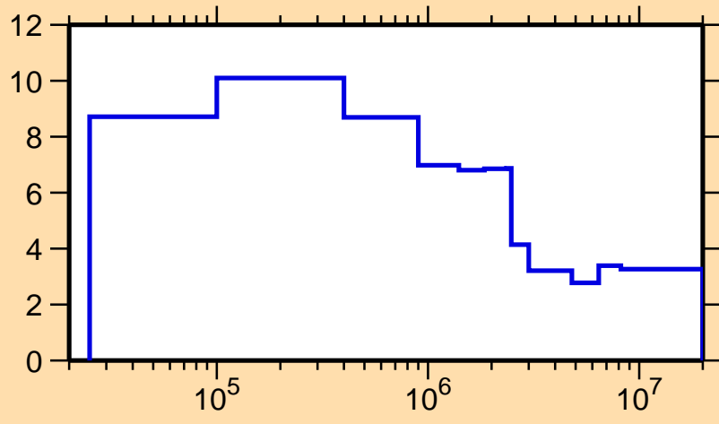
\Delta\sigma/\sigma vs. E for ^{71}\text{Se}(n,\text{nonel.})
