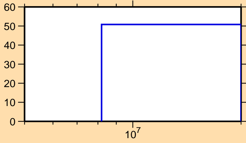
\Delta\sigma/\sigma vs. E for ^{71}\text{Se}(n,2n)
