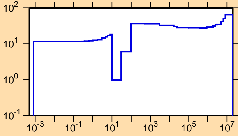
\Delta\sigma/\sigma vs. E for ^{71}\text{Se}(n,\gamma)
