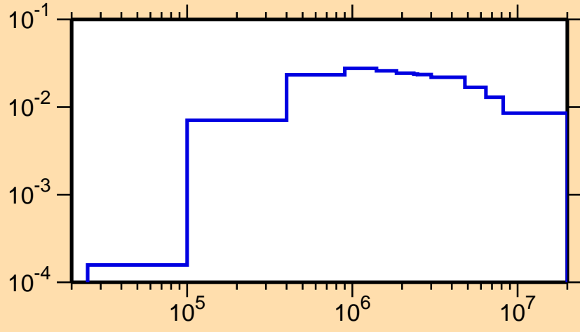
\sigma vs. E for ^{71}\text{Se}(n,n_1)
