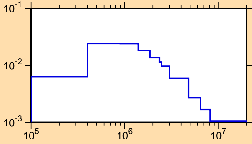
\sigma vs. E for ^{71}\text{Se}(n,n_2)
