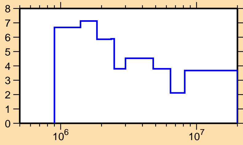
\Delta\sigma/\sigma vs. E for ^{71}\text{Se}(n,\text{el.})
