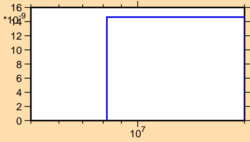
\sigma vs. E for ^{71}\text{Se} (mt 45)
