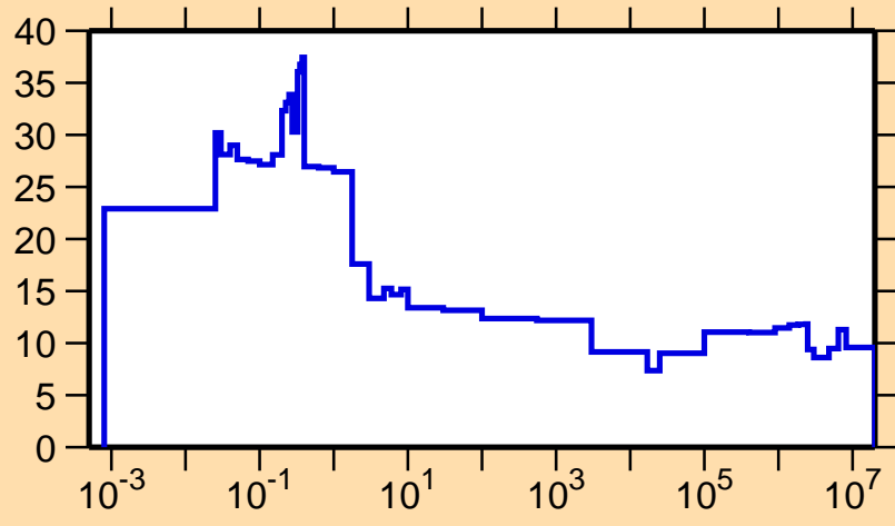
\Delta\sigma/\sigma vs. E for ^{71}\text{Se}(n,p)
