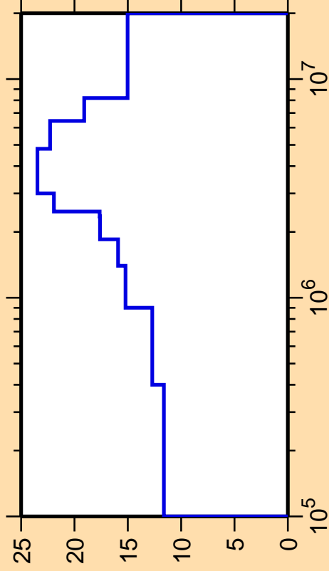
\Delta\sigma/\sigma vs. E for ^{71}\text{Se}(n,n_3)
