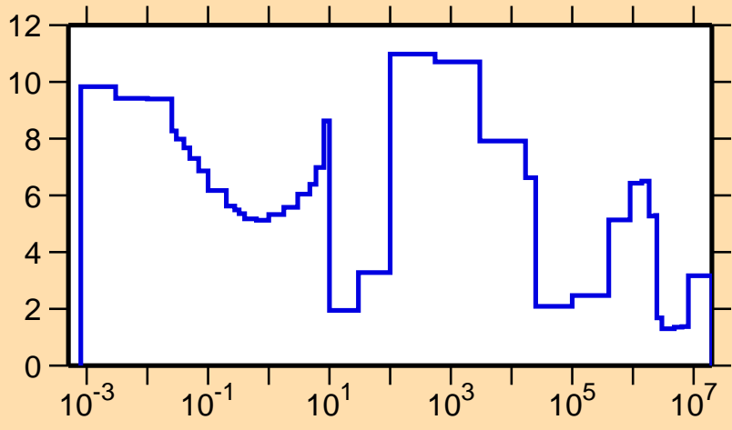
\Delta\sigma/\sigma vs. E for ^{71}\text{Se}(n,\text{tot.})
