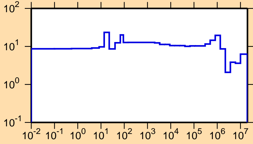
\Delta\sigma/\sigma vs. E for ^{73}\text{Se}(n,el.)
