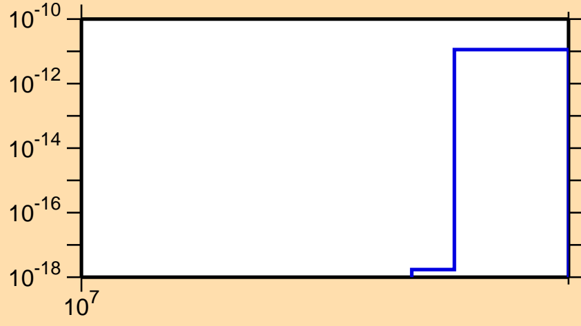
\sigma vs. E for ^{74}\text{Se} (mt 45)
