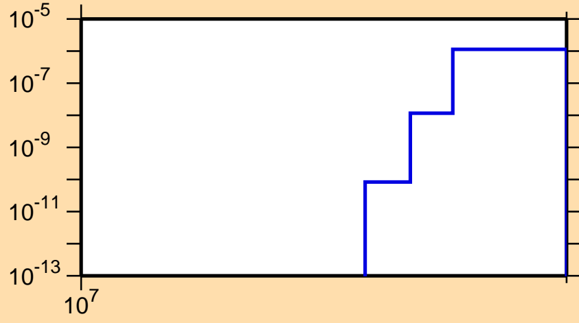
\sigma vs. E for ^{74}\text{Se}(n,pd)
