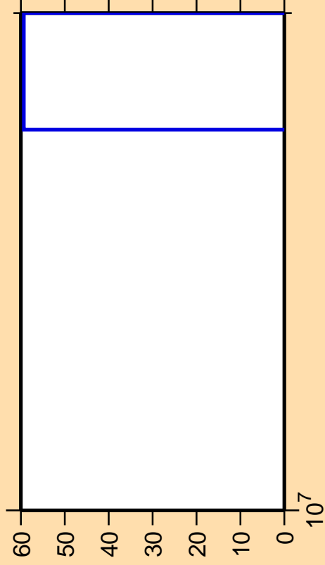
\Delta\sigma/\sigma vs. E for ^{74}\text{Se}(n,nd)
