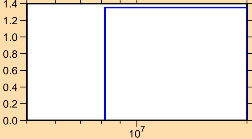
\Delta\sigma/\sigma vs. E for ^{74}\text{Se}(n,\text{tot.})
