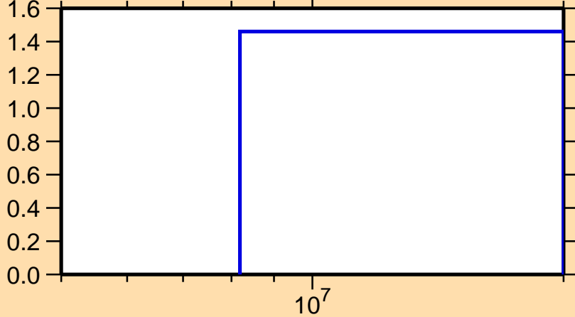
\Delta\sigma/\sigma vs. E for ^{74}\text{Se}(n,\text{nonel.})
