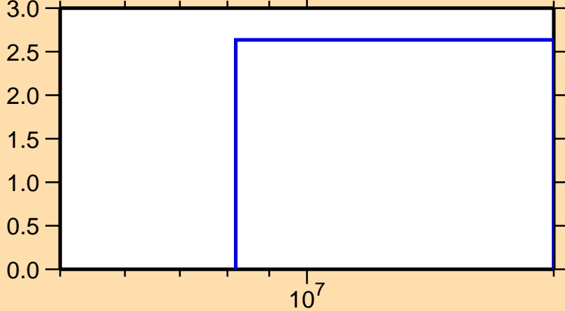
\Delta\sigma/\sigma vs. E for ^{74}\text{Se}(n,\text{inel.})
