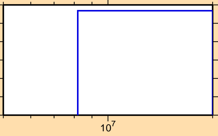
\sigma vs. E for ^{74}\text{Se}(n,p\alpha)
