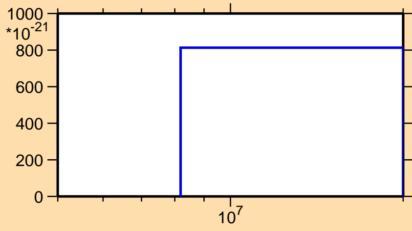
\sigma vs. E for ^{74}\text{Se}(n,nt)
