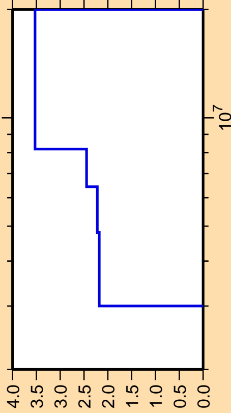
\Delta\sigma/\sigma vs. E for ^{74}\text{Se}(n,n\text{cont.})
