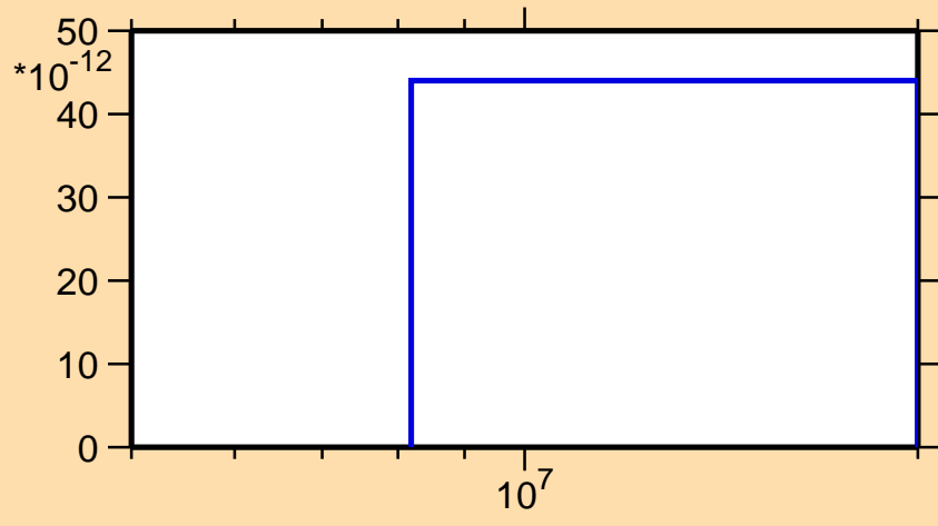
\sigma vs. E for ^{75}\text{Se}(n,\text{pd})
