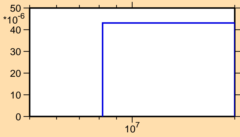
\sigma vs. E for ^{75}\text{Se}(n,t)
