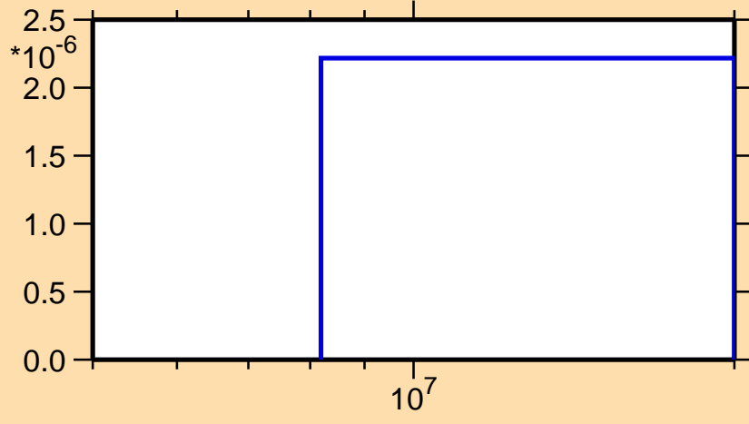
\sigma vs. E for ^{75}\text{Se}(n,p\alpha)
