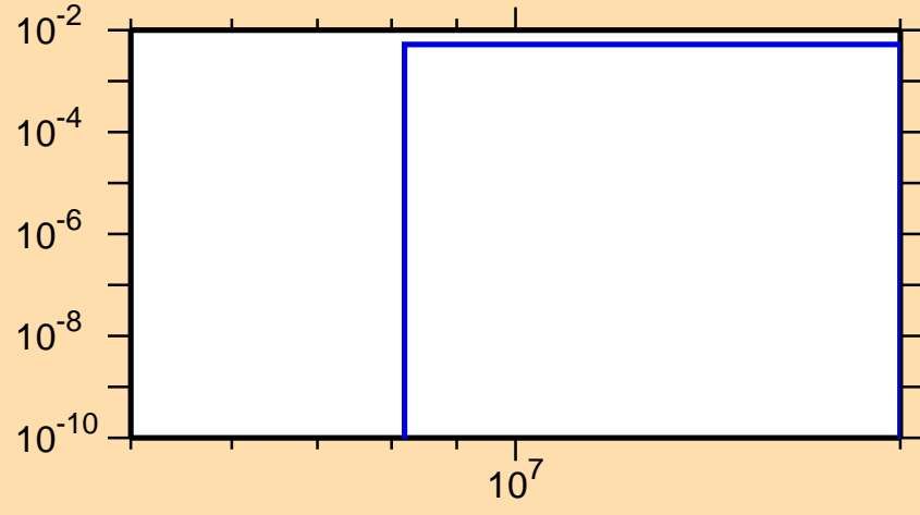
\sigma vs. E for ^{75}\text{Se}(n,n\alpha)
