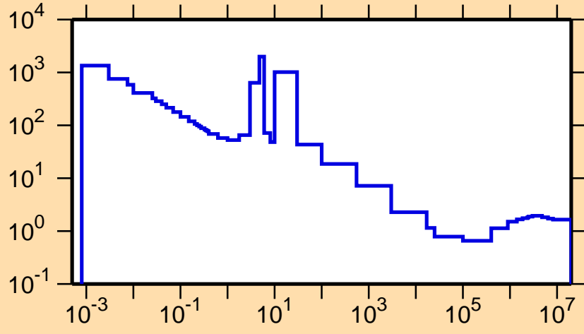
\sigma vs. E for ^{75}\text{Se}(n,\text{nonel.})
