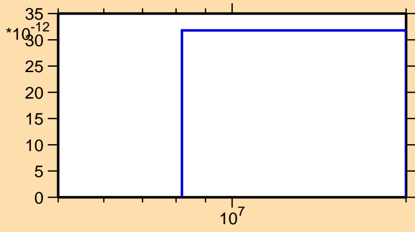
\sigma vs. E for ^{75}\text{Se}(n,\text{pt})
