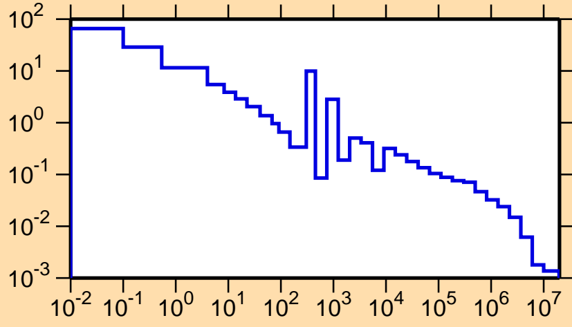
\sigma vs. E for ^{76}\text{Se}(n,\gamma)
