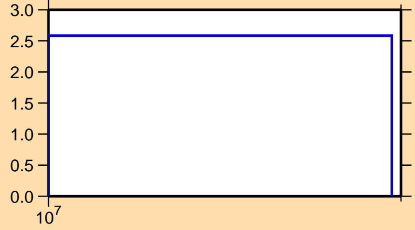
\Delta\sigma/\sigma vs. E for ^{76}\text{Se}(n,\text{inel.})
