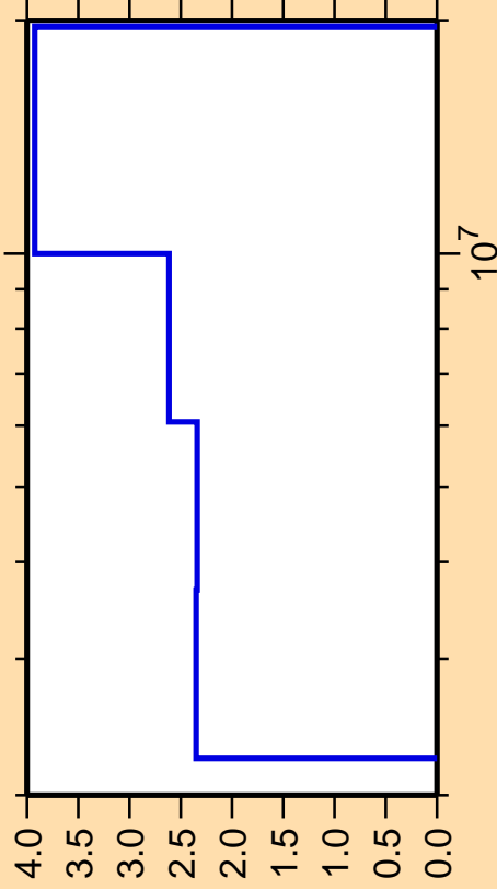
\Delta\sigma/\sigma vs. E for ^{76}\text{Se}(n,n_{\text{cont}}) .
