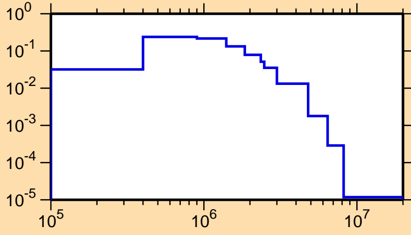
\sigma vs. E for ^{77}\text{Se}(n,n_4)
