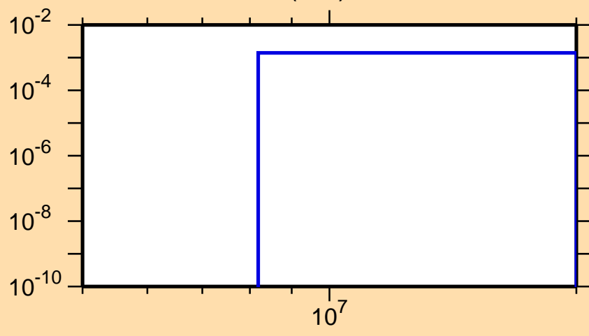
\sigma vs. E for ^{77}\text{Se}(n,d)
