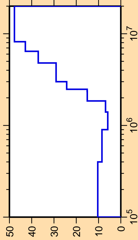
\Delta\sigma/\sigma vs. E for ^{77}\text{Se}(n,n_4)
