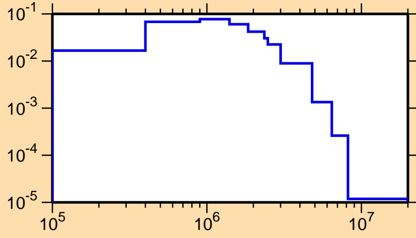
\sigma vs. E for ^{77}\text{Se}(n,n_1)
