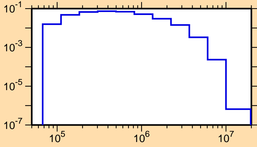
\sigma vs. E for ^{77}\text{Se}(n,n_3)
