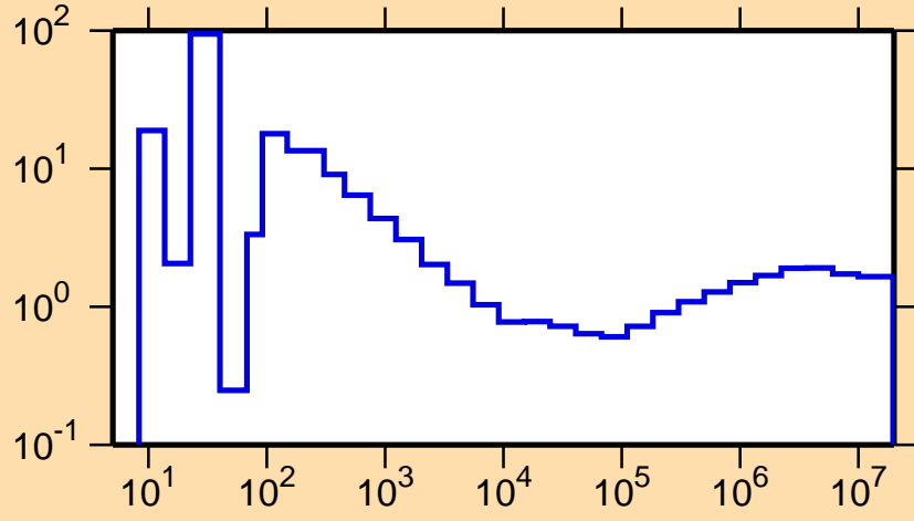
\sigma vs. E for ^{77}\text{Se}(n,\text{nonel.})
