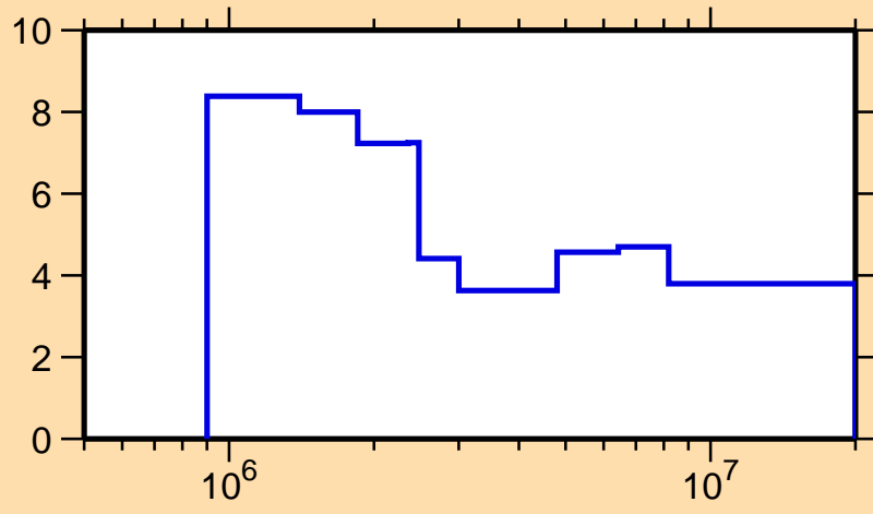
\Delta\sigma/\sigma vs. E for ^{77}\text{Se}(n,n\text{oncl.})
