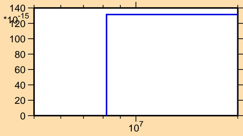
\sigma vs. E for ^{78}\text{Se}(n,nd)
