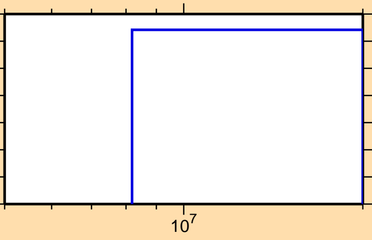
\sigma vs. E for ^{78}\text{Se}(n,3n)
