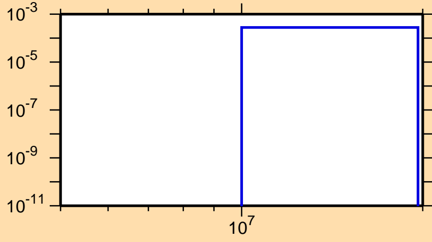
\sigma vs. E for ^{79}\text{Se}(n,n\alpha)
