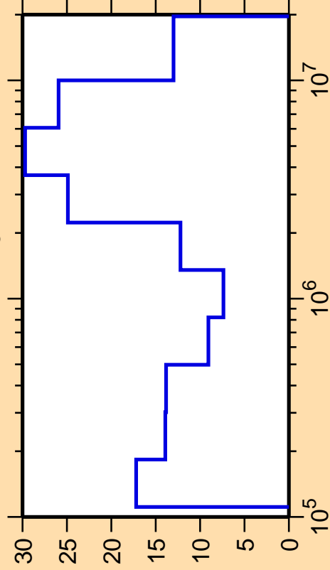
\Delta\sigma/\sigma vs. E for ^{79}\text{Se}(n,n_3)
