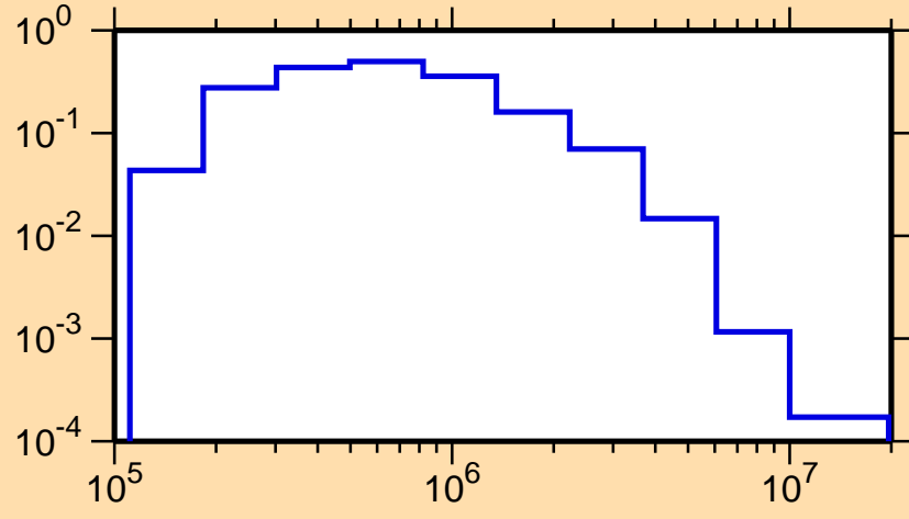
\sigma vs. E for ^{79}\text{Se}(n,n_3)
