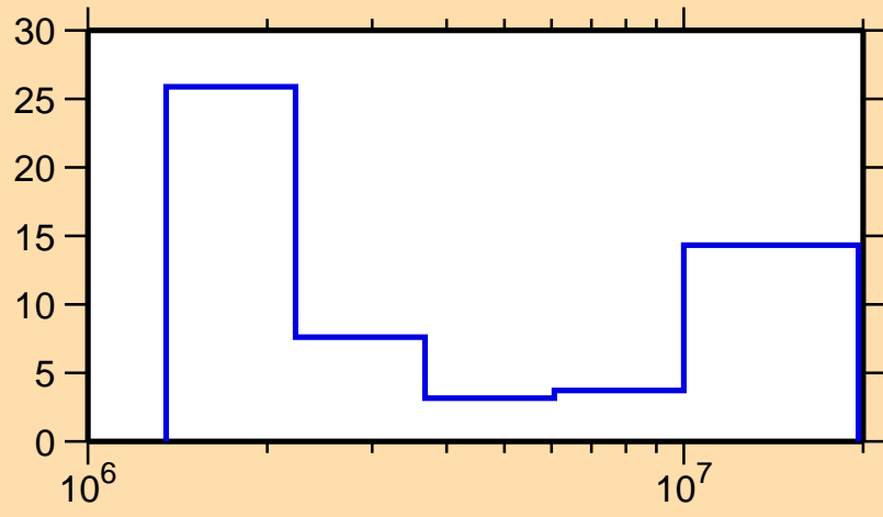
\Delta\sigma/\sigma vs. E for ^{79}\text{Se}(n,n\text{cont.})
