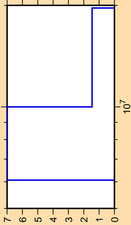
\Delta\sigma/\sigma vs. E for ^{79}\text{Se}(n,2n)
