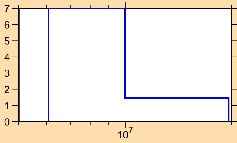
\Delta\sigma/\sigma vs. E for ^{79}\text{Se}(n,2n)
