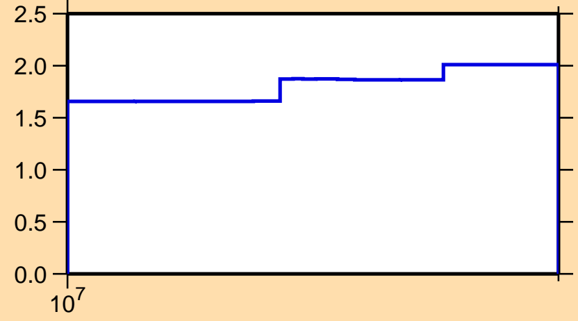
\Delta\sigma/\sigma vs. E for ^{80}\text{Se}(n,\text{nonel.})
