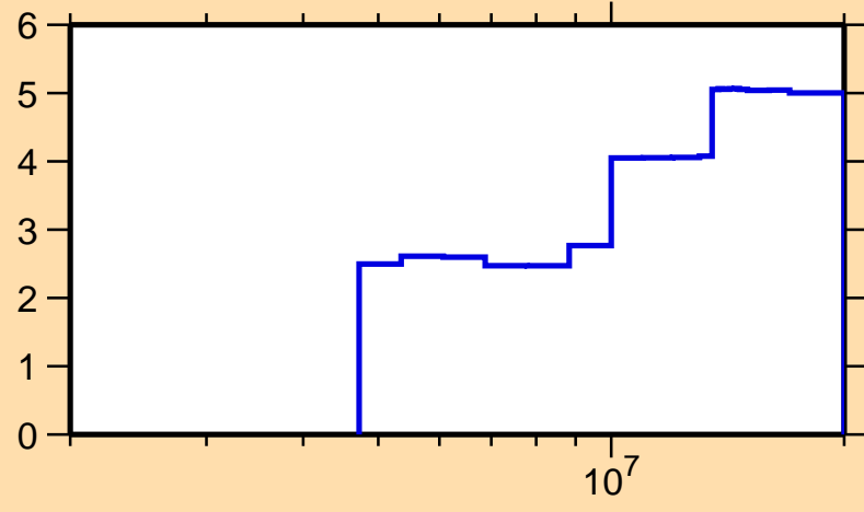
\Delta\sigma/\sigma vs. E for ^{80}\text{Se}(n,n\text{cont.})
