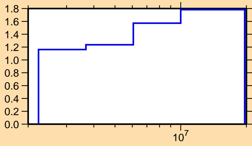
\Delta\sigma/\sigma vs. E for ^{80}\text{Se}(n,n\text{nonel.})
