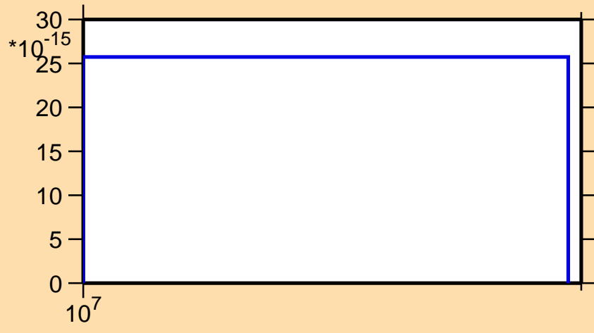
\sigma vs. E for ^{80}\text{Se}(n,\text{He}3)
