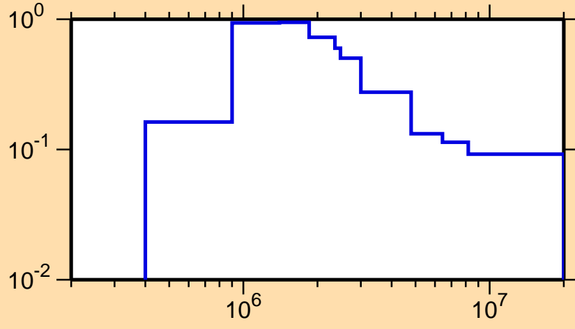
\sigma vs. E for ^{80}\text{Se}(n,n_1)
