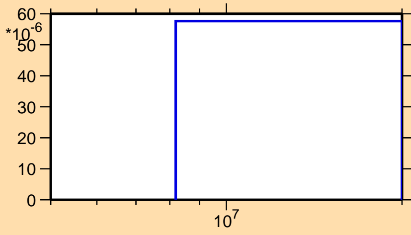
\sigma vs. E for ^{80}\text{Se}(n,n\alpha)
