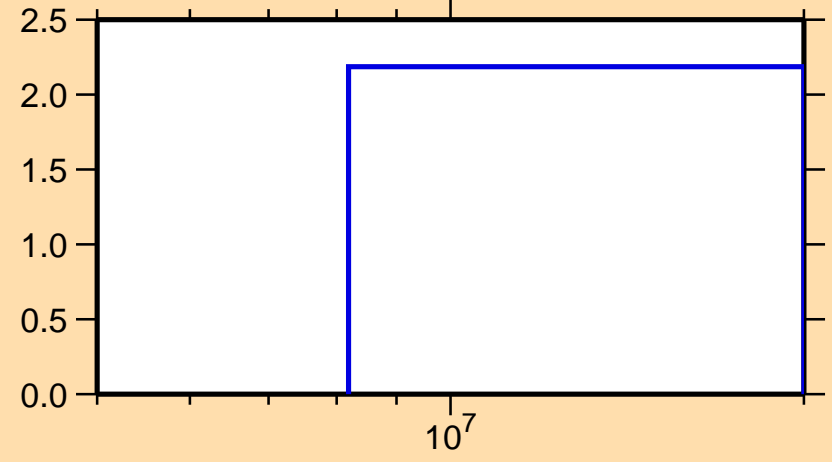
\Delta\sigma/\sigma vs. E for ^{80}\text{Se}(n,\text{el.})
