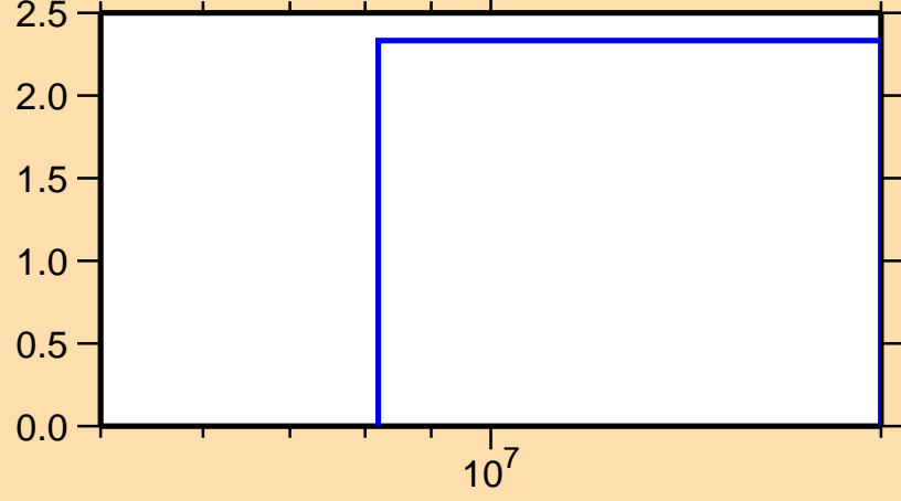
\Delta\sigma/\sigma vs. E for ^{80}\text{Se}(n,\text{inel.})
