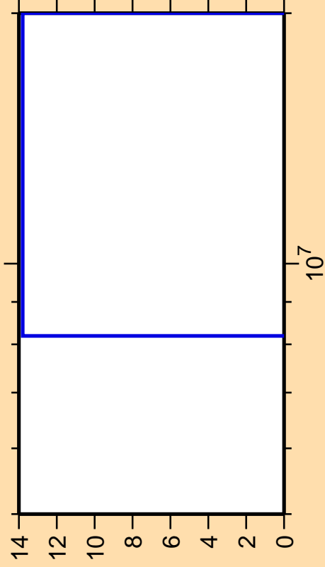
\Delta\sigma/\sigma vs. E for ^{80}\text{Se}(n,n\alpha)
