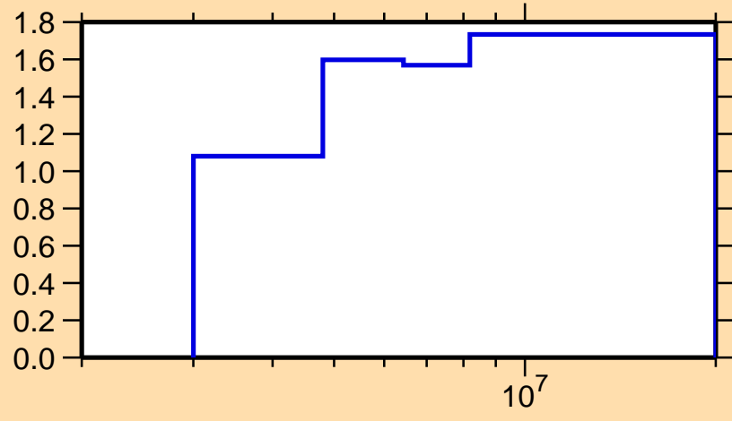
\Delta\sigma/\sigma vs. E for ^{80}\text{Se}(n,n\text{onel.})
