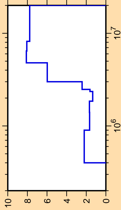
\Delta\sigma/\sigma vs. E for ^{80}\text{Se}(n,n_1)
