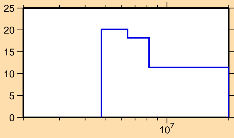
\Delta\sigma/\sigma vs. E for ^{80}\text{Se}(n,p)
