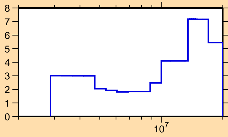
\Delta\sigma/\sigma vs. E for ^{81}\text{Se}(n,el.)
