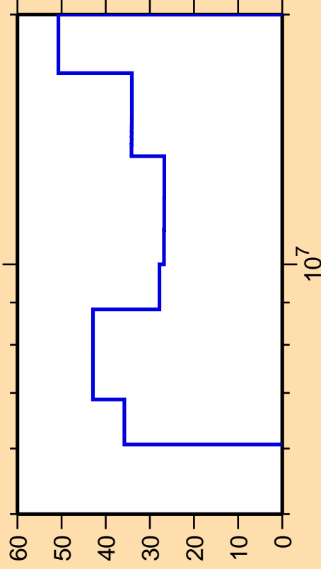
\Delta\sigma/\sigma vs. E for ^{81}\text{Se}(n,\alpha)
