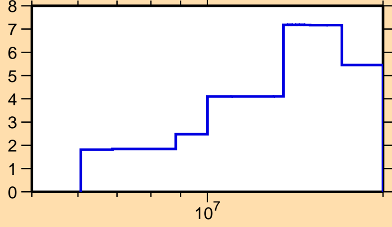
\Delta\sigma/\sigma vs. E for ^{81}\text{Se}(n,\text{el.})
