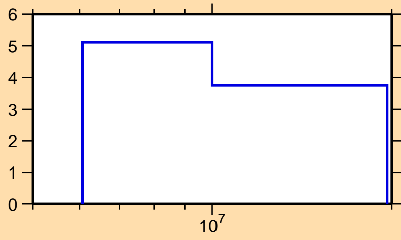
\Delta\sigma/\sigma vs. E for ^{81}\text{Se}(n,2n)
