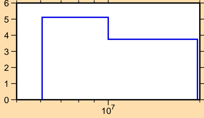
\Delta\sigma/\sigma vs. E for ^{81}\text{Se}(n,2n)
