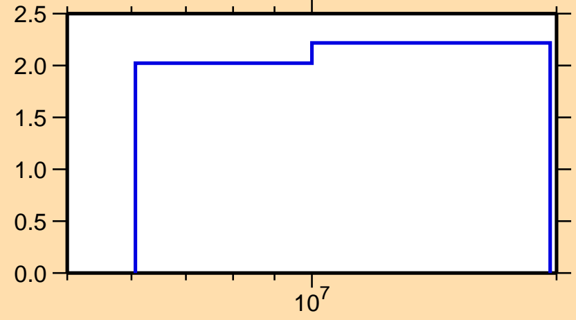
\Delta\sigma/\sigma vs. E for ^{81}\text{Se}(n,\text{nonel.})
