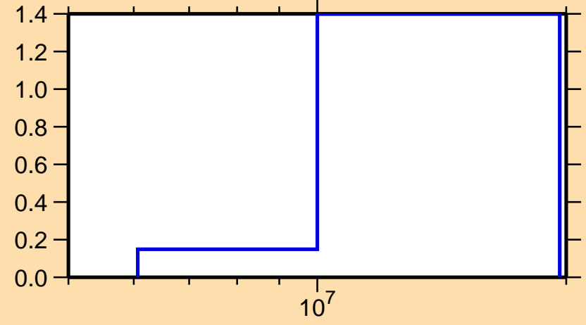
\sigma vs. E for ^{81}\text{Se}(n,2n)
