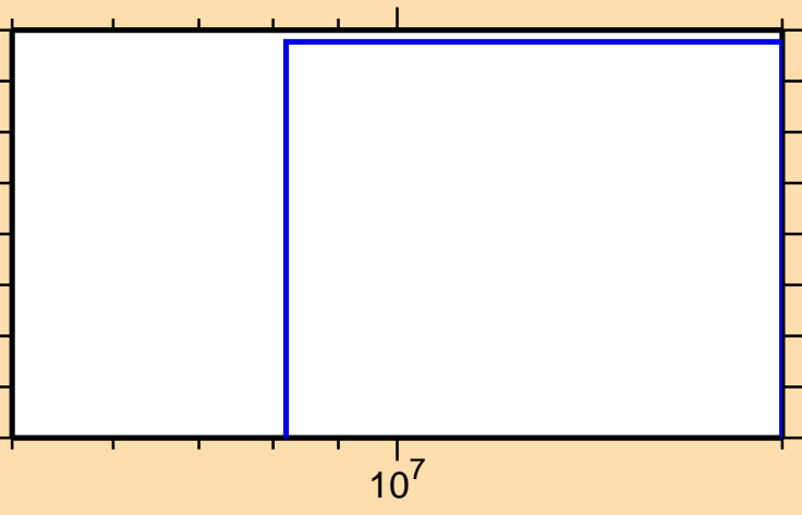
\sigma vs. E for ^{81}\text{Se}(n,np)
