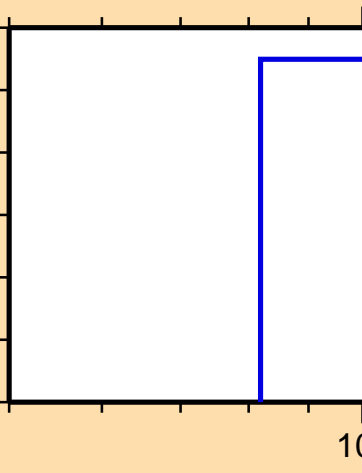
\sigma vs. E for ^{81}\text{Se}(\text{mt } 34)
