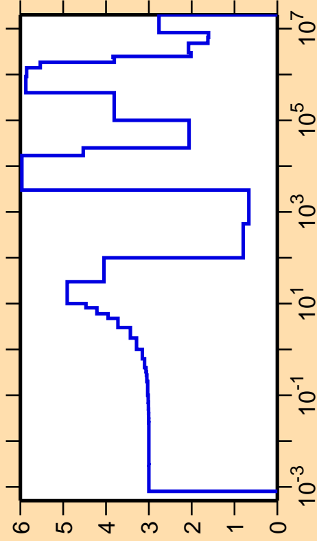
\Delta\sigma/\sigma vs. E for ^{81}\text{Se}(n,\text{el.})
