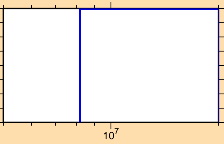
\sigma vs. E for ^{81}\text{Se}(n,3n)
