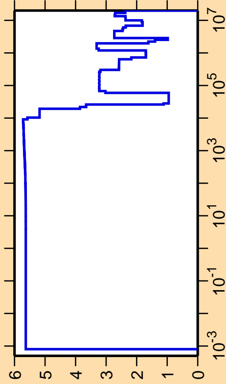
\Delta\sigma/\sigma vs. E for ^{82}\text{Se}(n,\text{el.})
