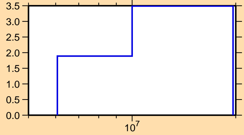
\Delta\sigma/\sigma vs. E for ^{82}\text{Se}(n,\text{inel.})
