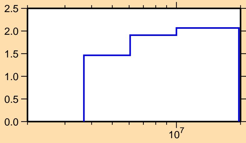
\Delta\sigma/\sigma vs. E for ^{82}\text{Se}(n,n\text{onrel.})
