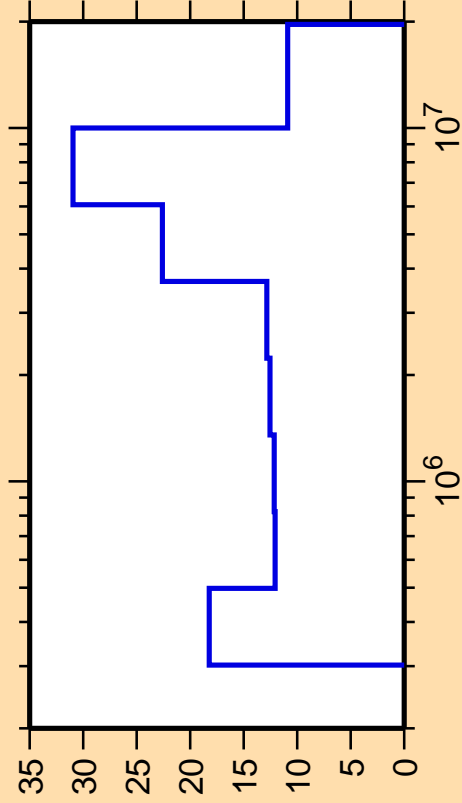
\Delta\sigma/\sigma vs. E for ^{83}\text{Se}(n,n_3)
