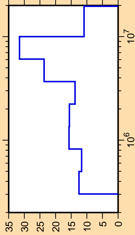
\Delta\sigma/\sigma vs. E for ^{83}\text{Se}(n,n_2)
