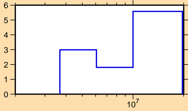
\Delta\sigma/\sigma vs. E for ^{83}\text{Se}(n,el.)
